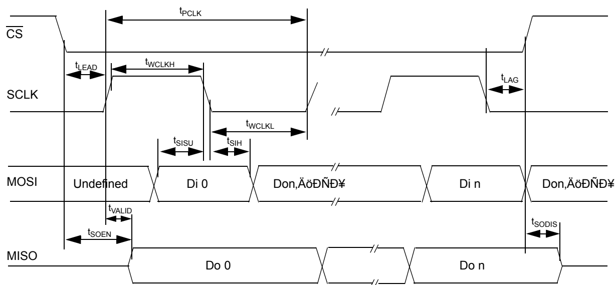
Figure 16. SPI Timings
