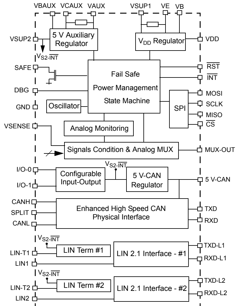
Figure 7. 33905D Internal Block Diagram
