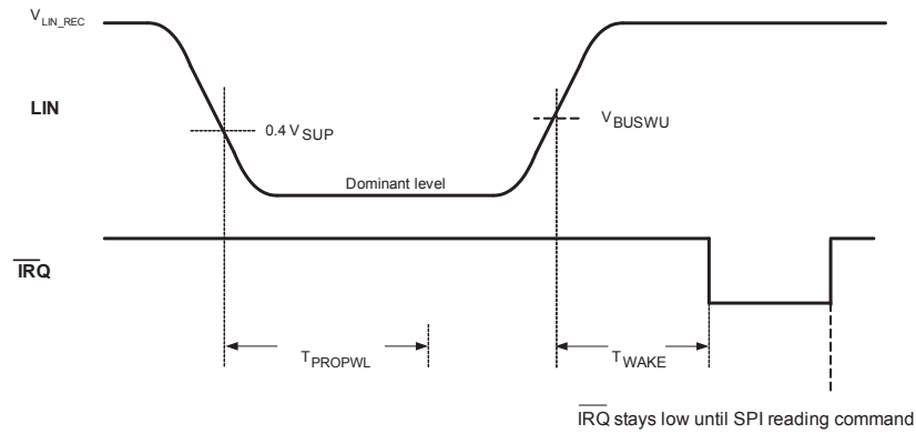
Figure 23. LIN Wake-up LP V DD ON Mode Timing
