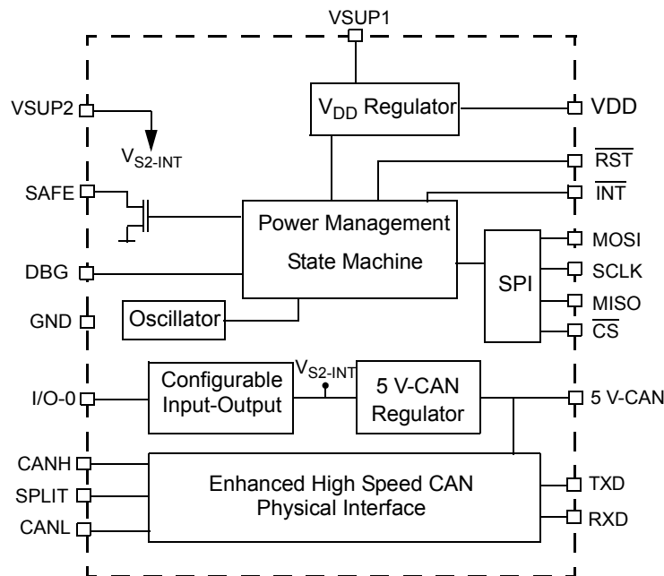
Figure 10. 33903 Internal Block Diagram
