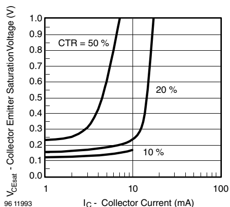
Fig. 9 - Collector Emitter Saturation Voltage vs. Collector Current
