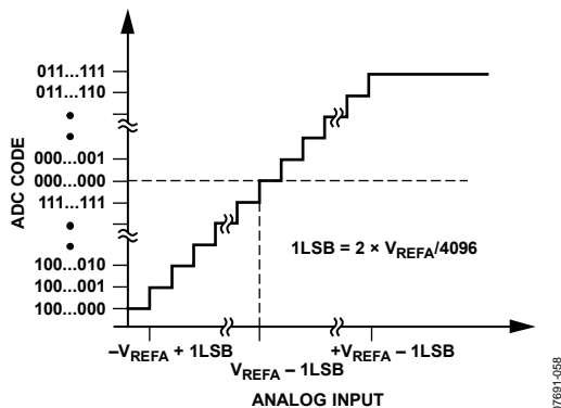
Figure 58. Twos Complement Transfer Characteristic with V_{\text{REFA}} \pm V_{\text{REFA}} Input Range
