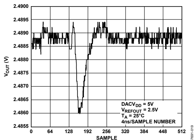
Figure 19. DAC-to-DAC Crosstalk
