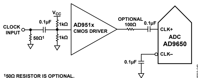
Figure 91. Single-Ended 1.8 V CMOS Input Clock (Up to 200 MHz)
