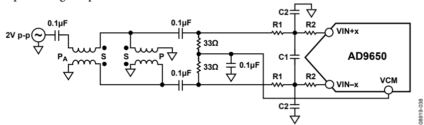
Figure 81. Differential Double Balun Input Configuration
