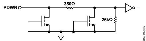
Figure 76. Equivalent PDWN Input Circuit
