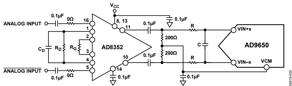
Figure 82. Differential Input Configuration Using the AD8352
