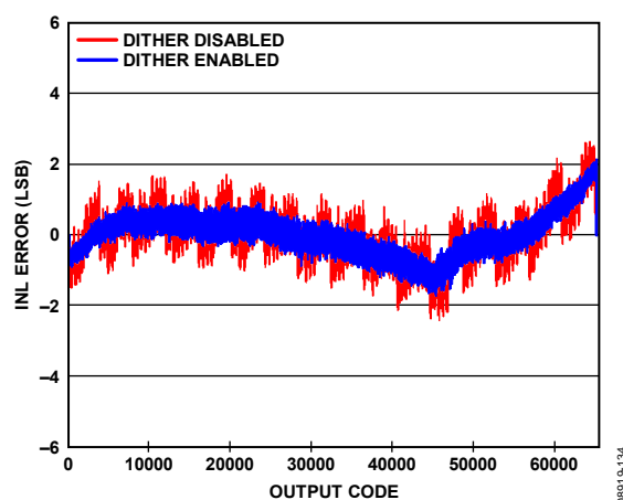
Figure 32. AD9650-65 INL with f_{IN} = 9.7 MHz
