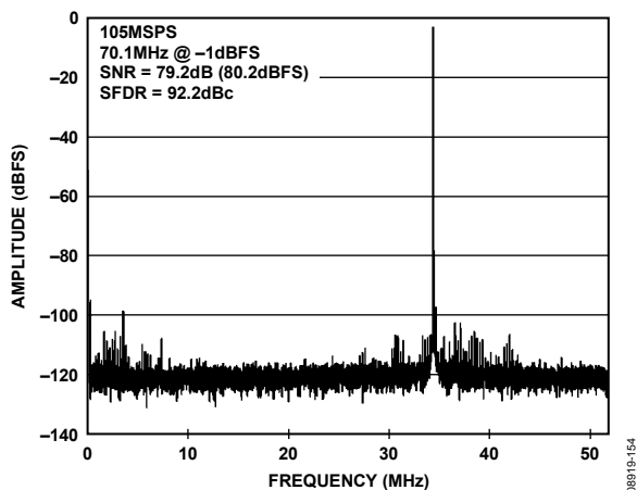
Figure 51. AD9650-105 Single-Tone FFT with f_{IN} = 70.1 MHz
