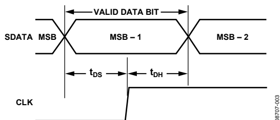
Figure 3. \overline{SDATA} Timing
