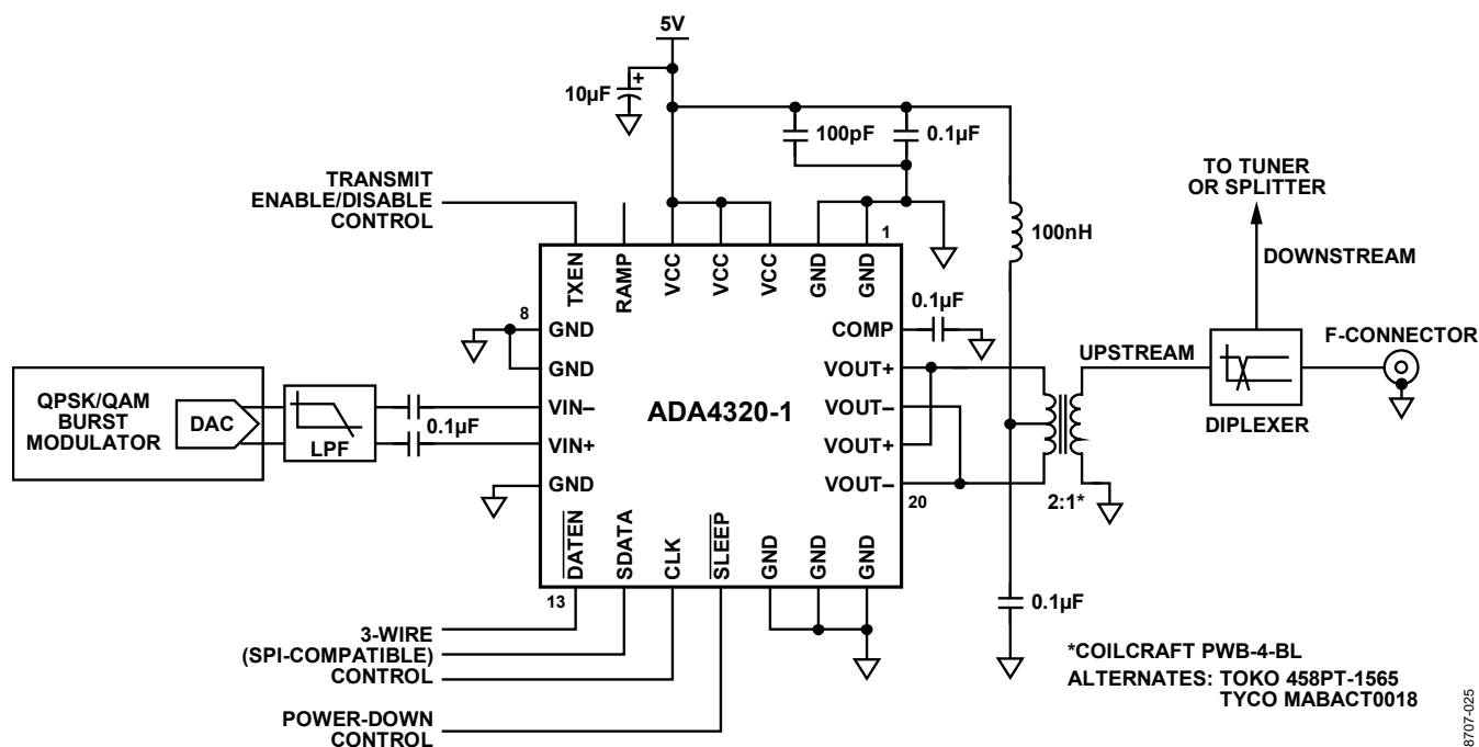
Figure 24. Typical Application
