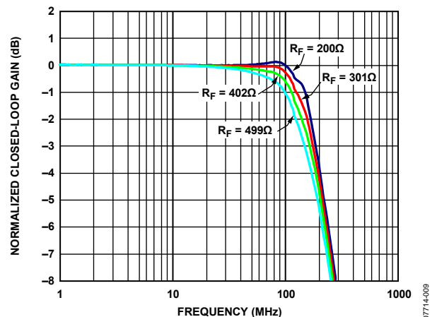
Figure 9. Large Signal Frequency Response vs. Feedback Resistor
