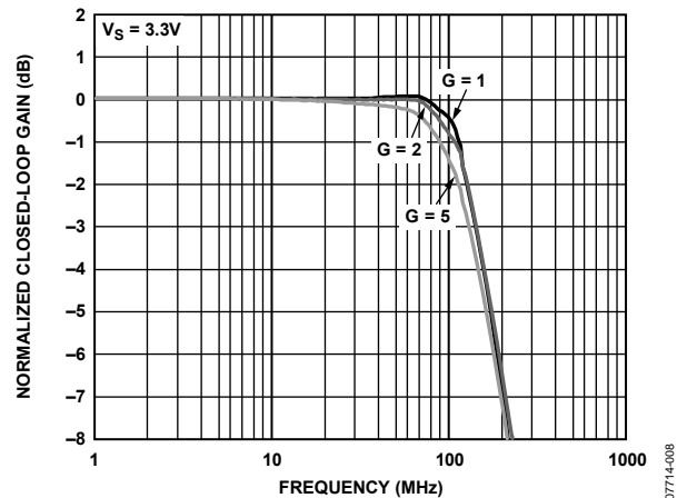
Figure 8. Large Signal Frequency Response vs. Gain
