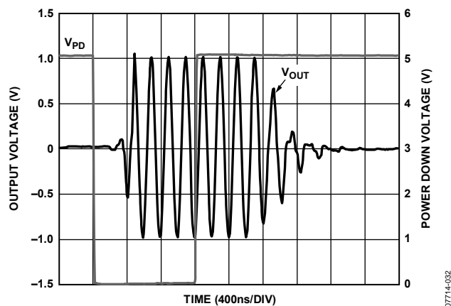
Figure 32. Enable/Power Down Time
