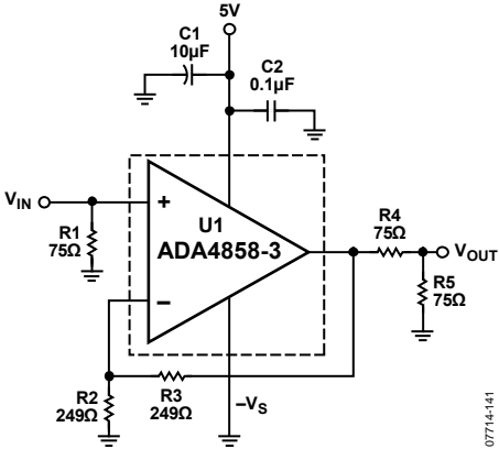
Figure 40. DC-Coupled, Single-Supply Schematic
