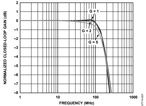
Figure 7. Large Signal Frequency Response vs. Gain
