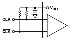
Figure 32. Use of the V_{REF} to Provide Low Impedance Termination into V_S/2
