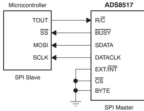
Figure 44. ADS8517 as SPI Master
