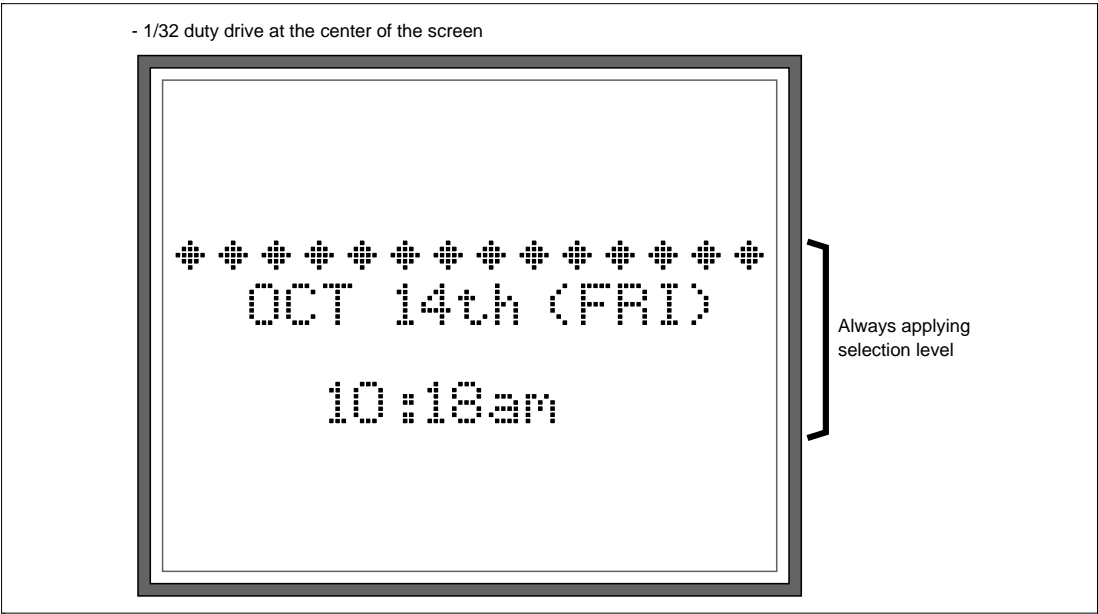
Figure 39 Partial-on Display (Date and Time Indicated) (2)
