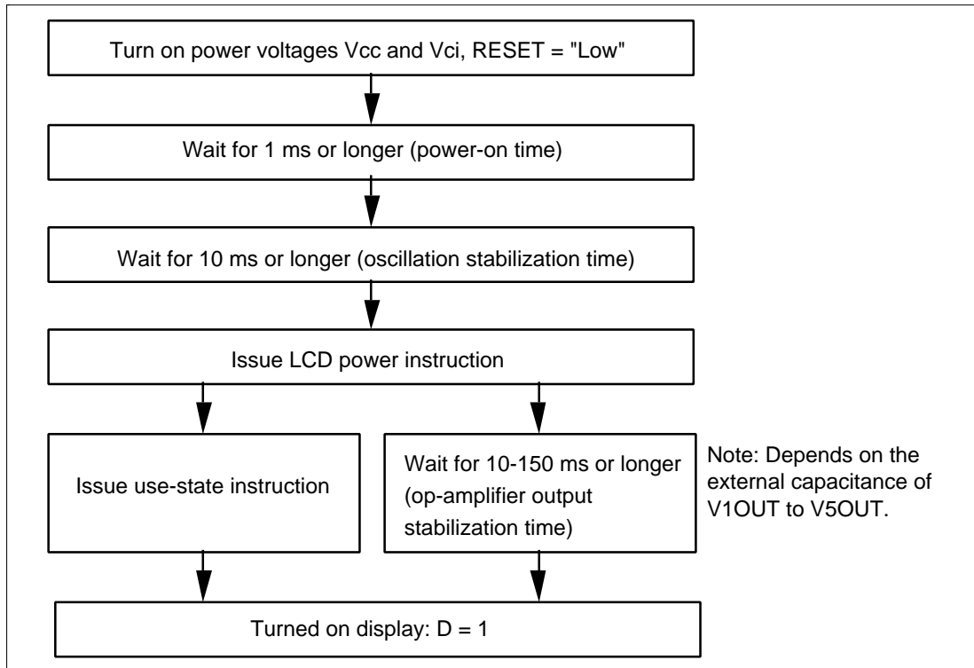
Figure 52 Power-on Sequence
