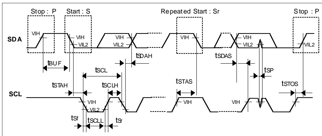
Figure 51 I2C bus Interface Timing
