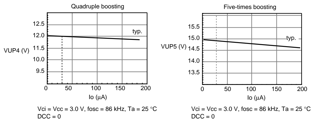
Figure 45 Booster (cont)
