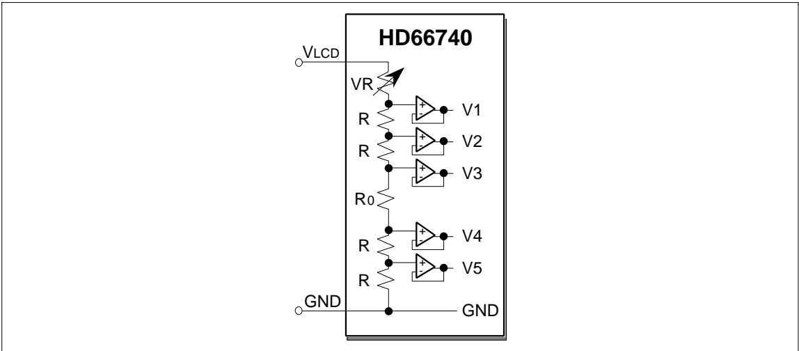
Figure 5 Contrast Adjuster
