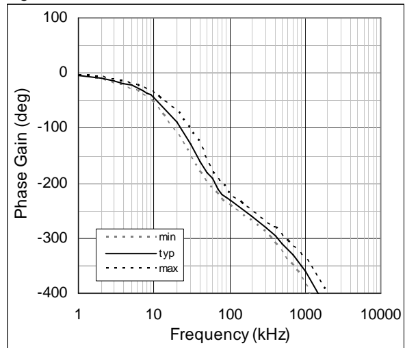
Figure 8. Phase Gain
