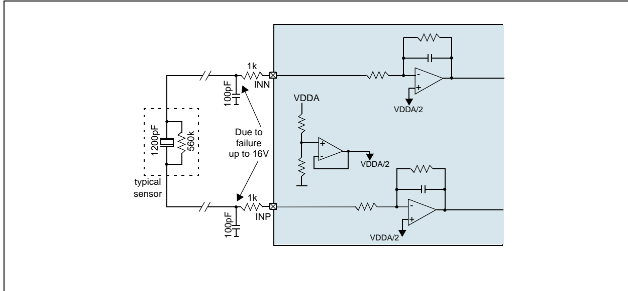
Figure 9. Sensor Biasing
