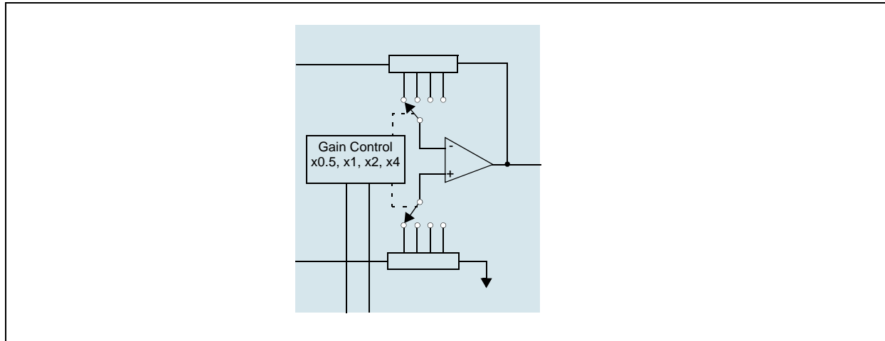
Figure 11. Subtractor Block
