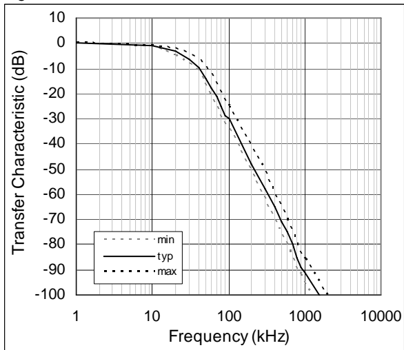
Figure 7. Transfer Characteristics
