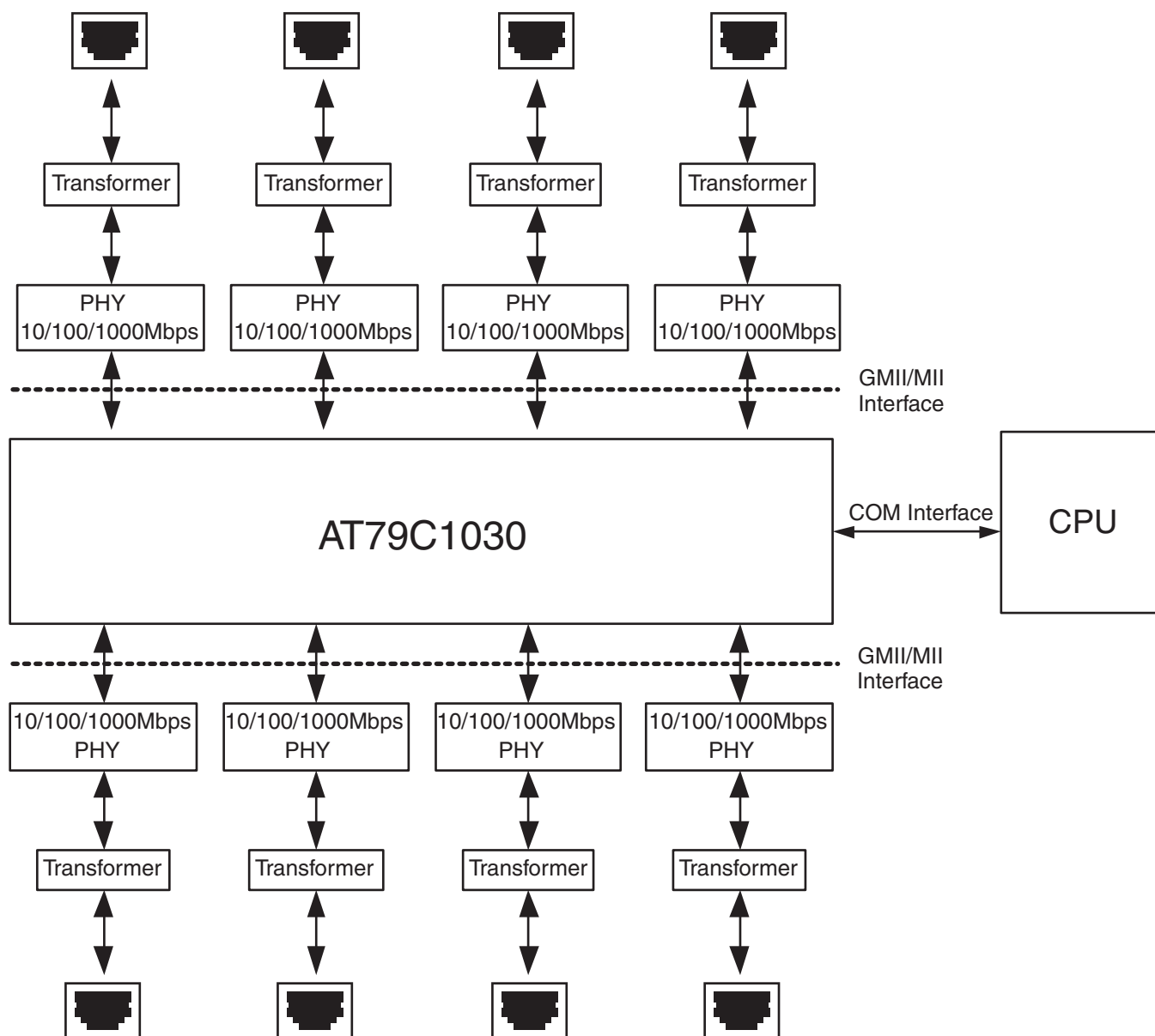
Figure 2. Application Diagram
