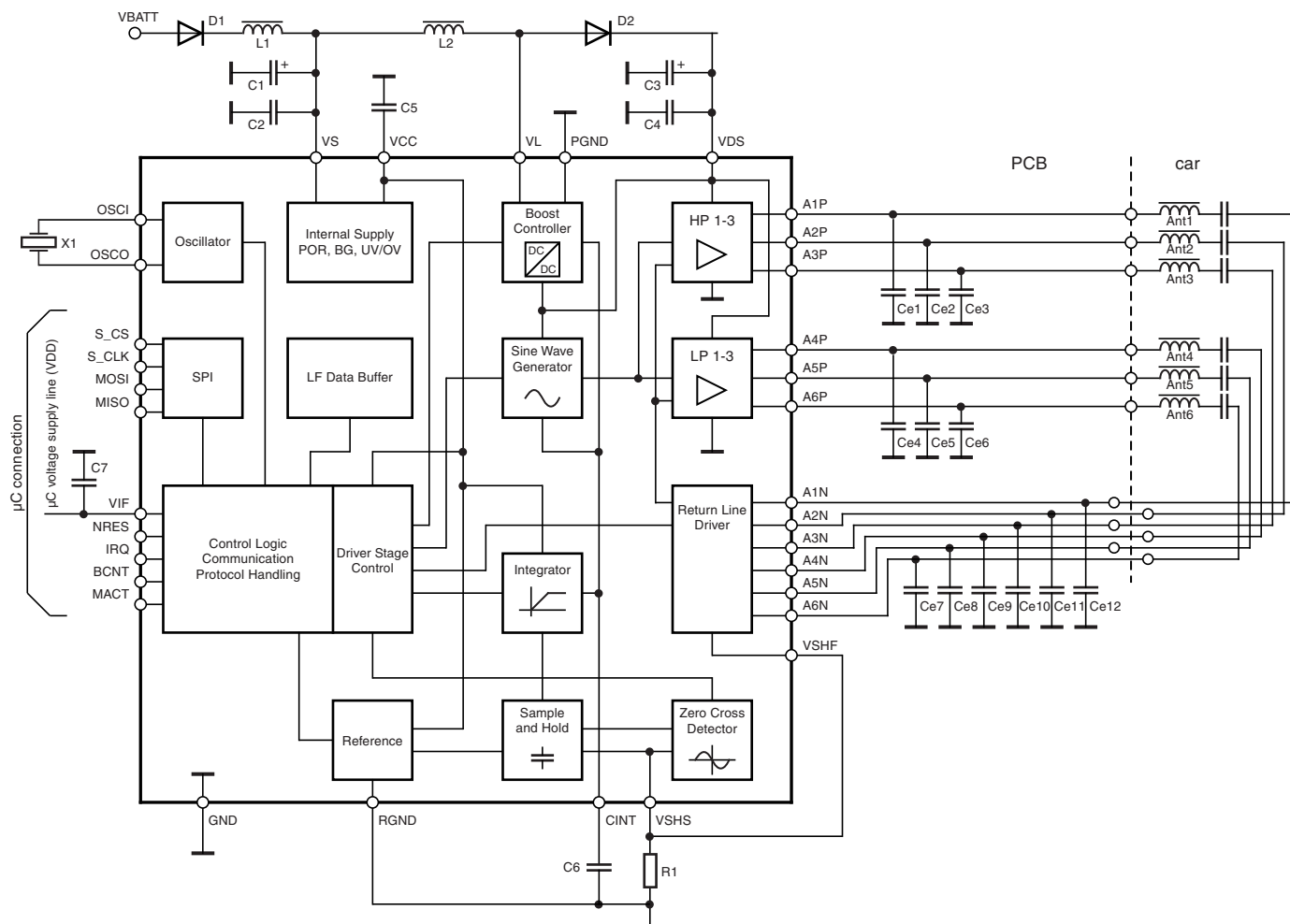
Figure 4-1. Application Schematic for ATA5279
