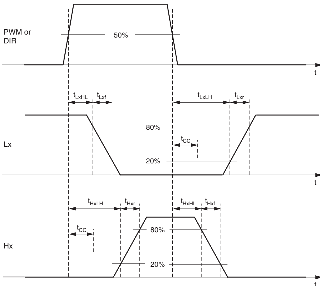
Figure 5-5. Timing of the Drivers
