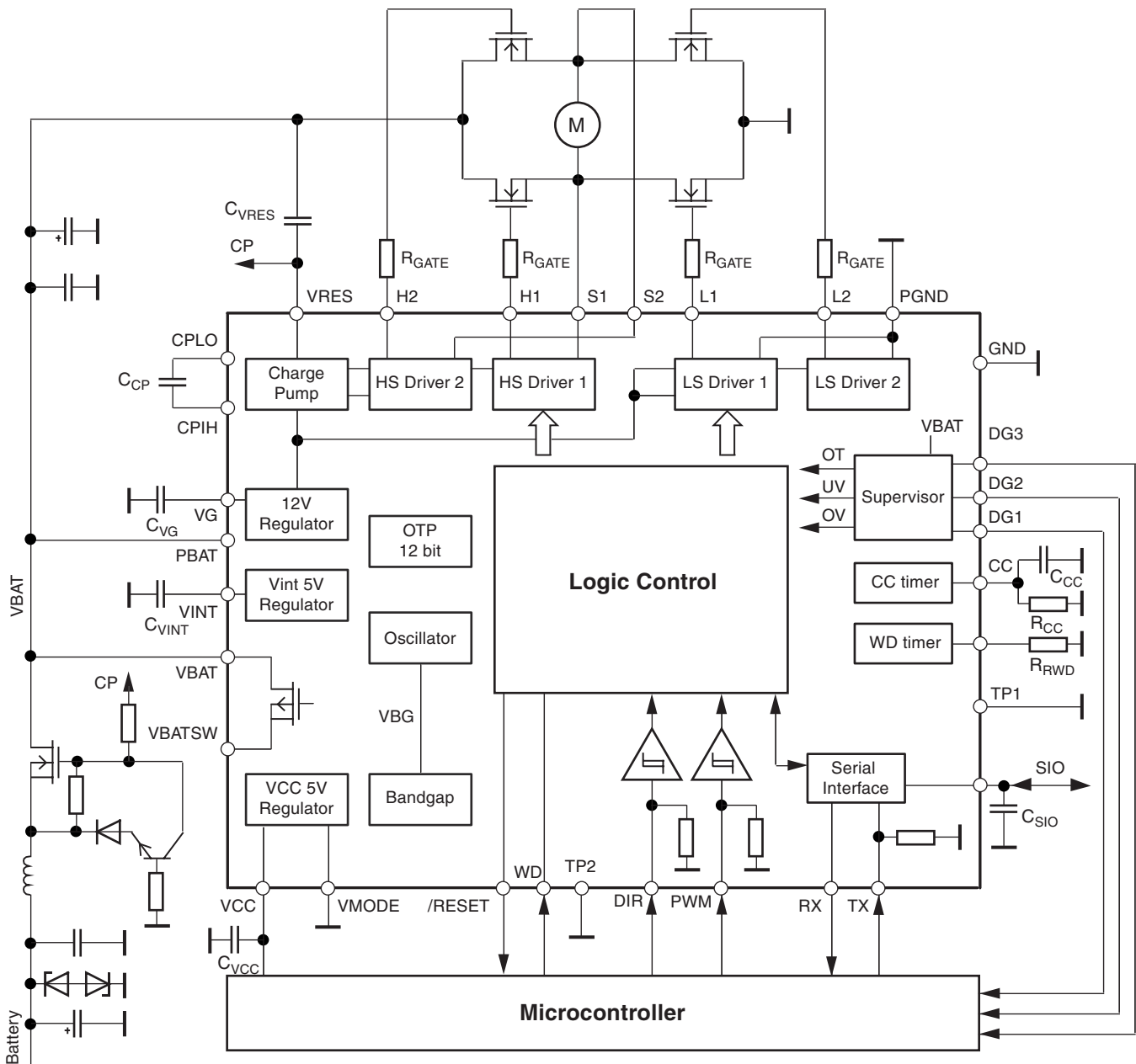
Figure 1-1. Block Diagram
