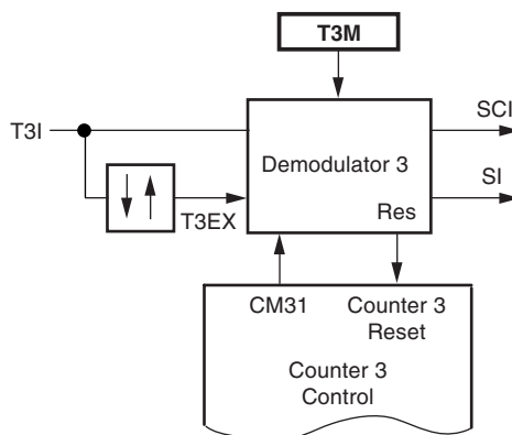
Figure 5-36. Timer 3 – Demodulator 3
