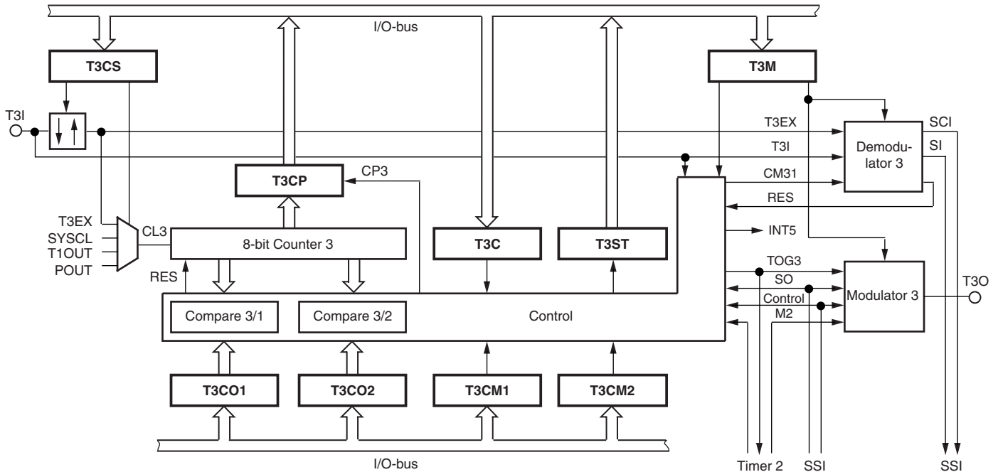
Figure 5-23. Timer 3
