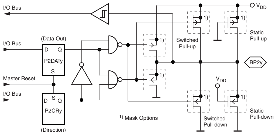
Figure 5-3. Bidirectional Port 2
