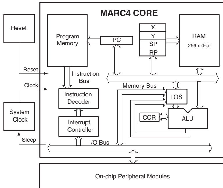
Figure 4-1. MARC4 Core
