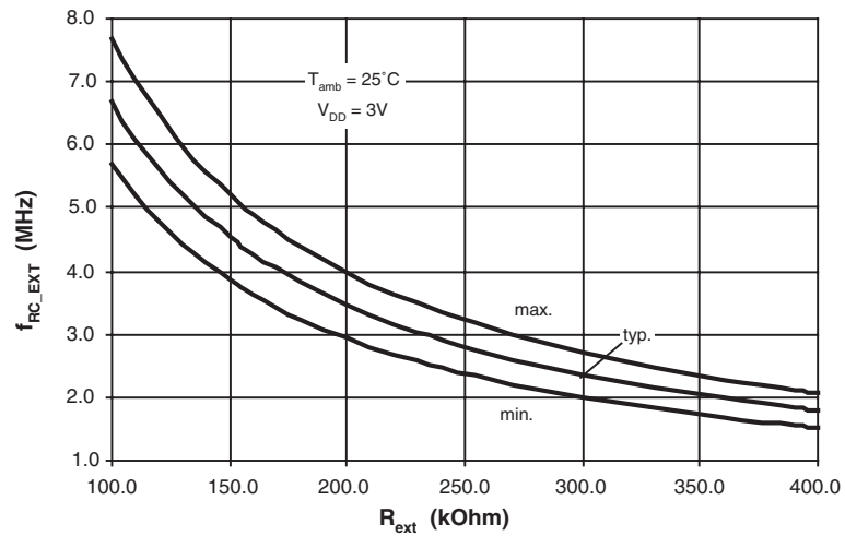
Figure 13-13. External RC Frequency versus R_{ext}
