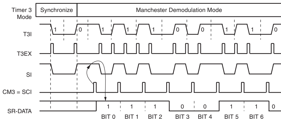
Figure 5-32. Timer 3 – Manchester Demodulation
