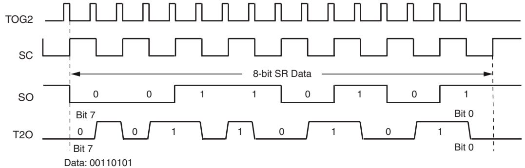
Figure 5-20. Manchester Modulation
