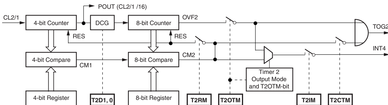
Figure 5-11. 12-bit Compare Counter
