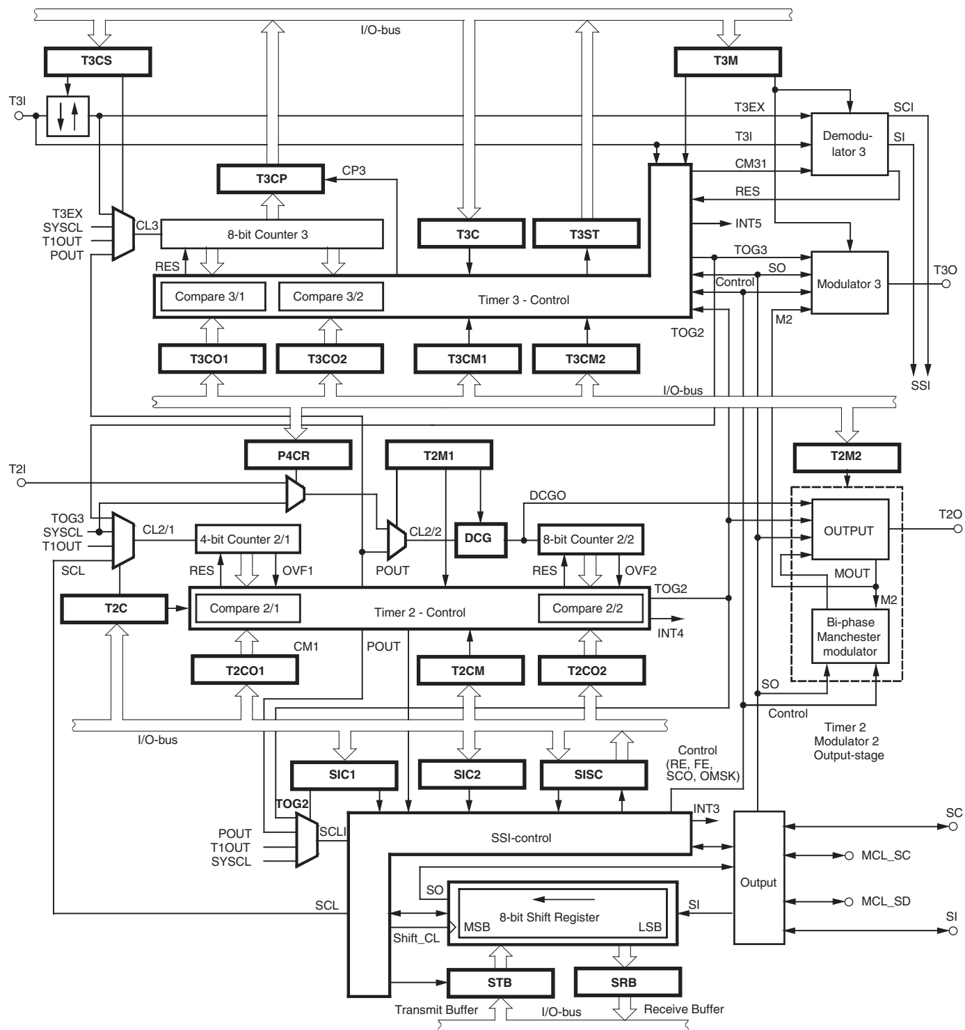
Figure 5-62. Combination Timer 2, Timer 3 and SSI
