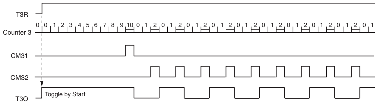
Figure 5-27. Single Action of Compare Register 1
