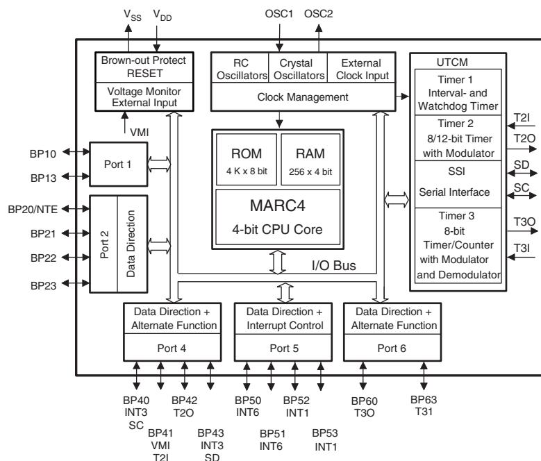
Figure 1-1. Block Diagram
