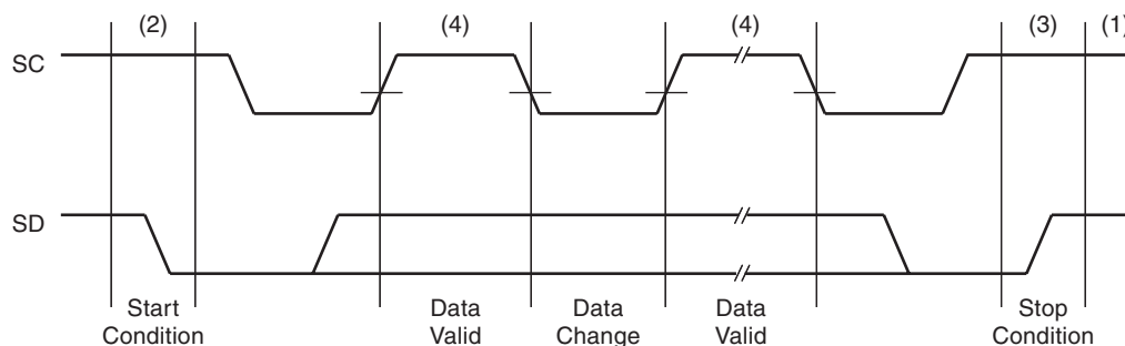
Figure 5-43. MCL Bus Protocol 1
