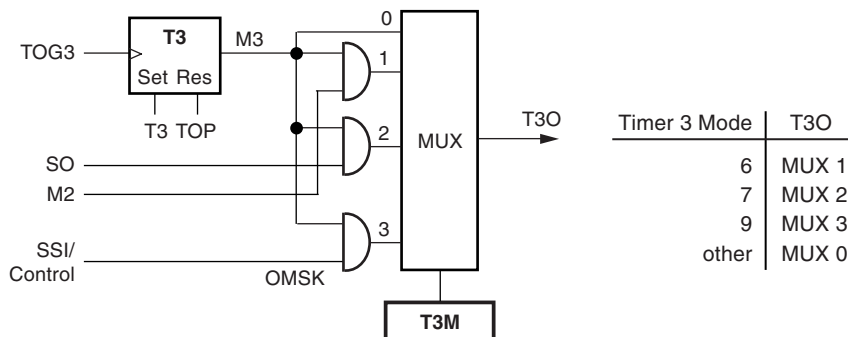
Figure 5-35. Modulator 3
