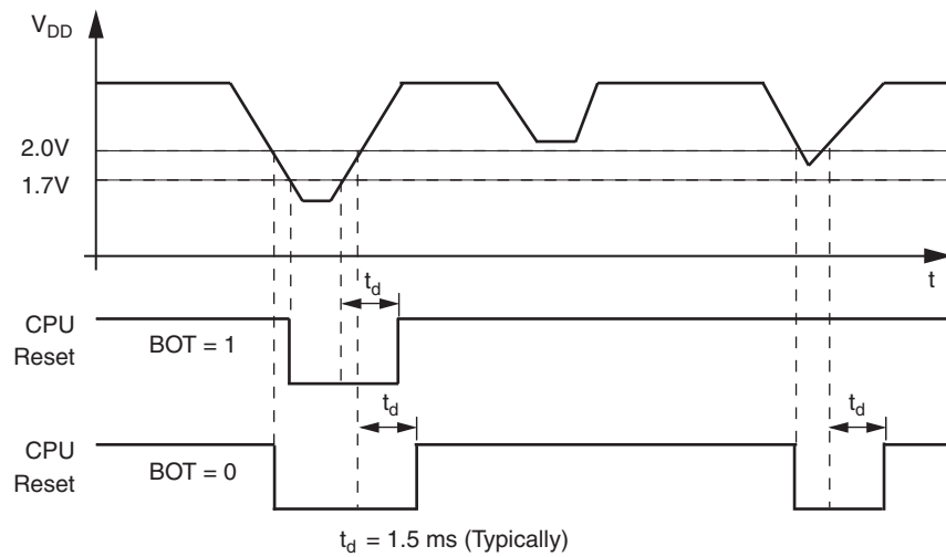
Figure 4-8. Brown-out Detection
