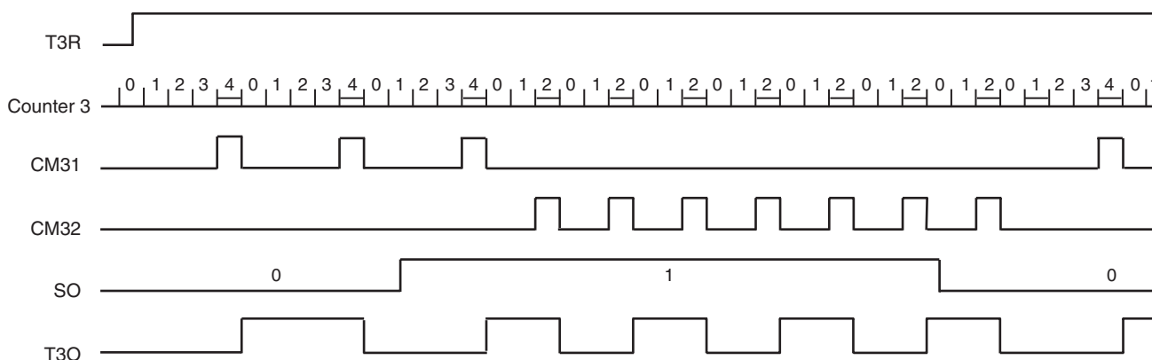
Figure 5-64. FSK Modulation
