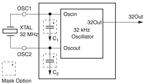
Figure 4-18. 32-kHz Crystal Oscillator
