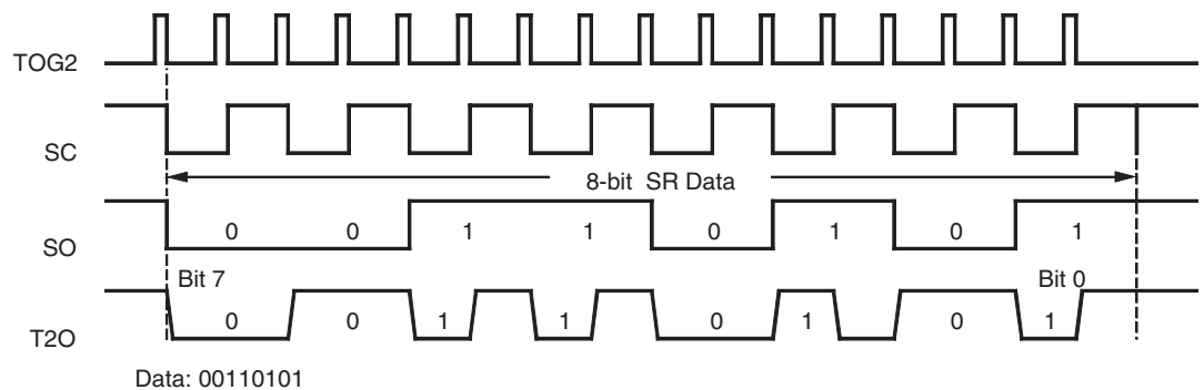
Figure 5-49. Bi-phase Modulation 1
