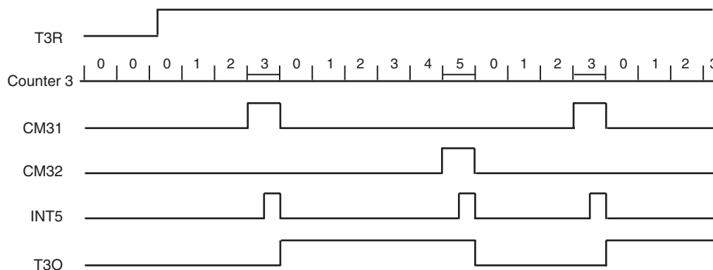
Figure 5-25. Counter Reset with Each Compare Match
