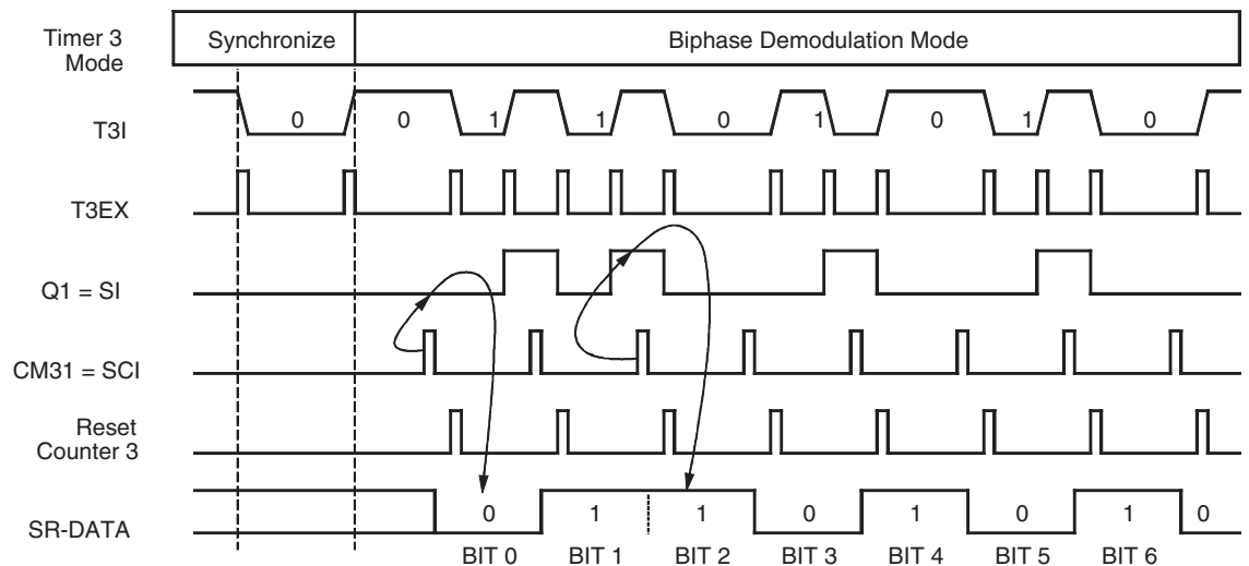
Figure 5-57. Bi-phase Demodulation
