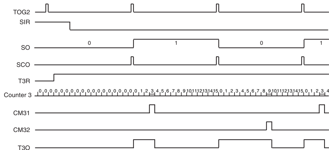
Figure 5-31. Pulse-width Modulation
