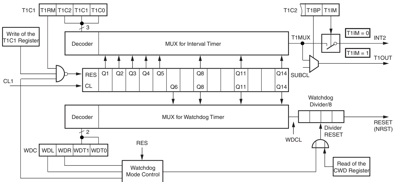
Figure 5-9. Timer 1 and Watchdog
