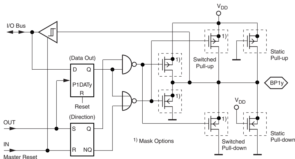
Figure 5-2. Bidirectional Port 1
