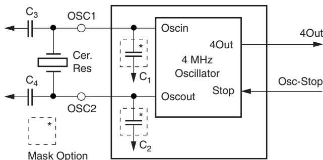
Figure 4-17. Ceramic Resonator
