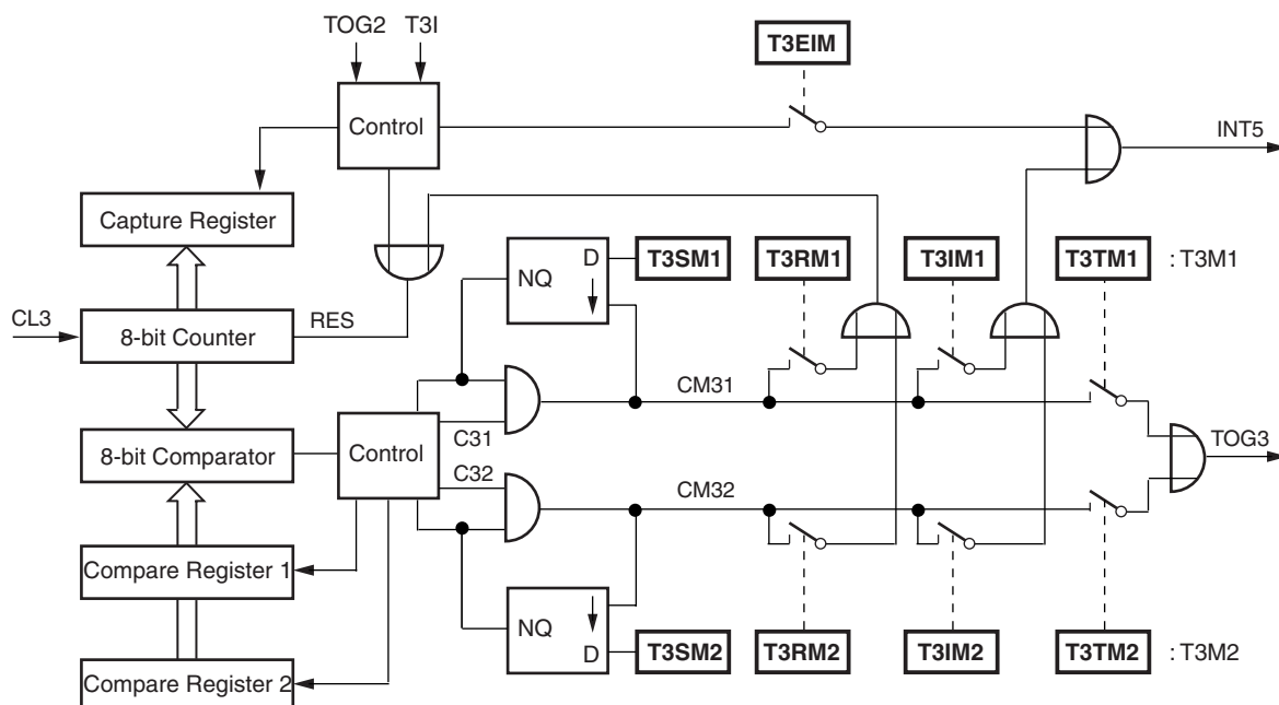
Figure 5-24. Counter 3 Stage
