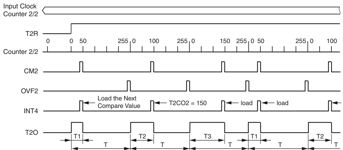
Figure 5-21. PWM Modulation
