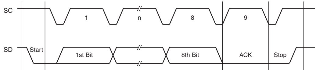
Figure 5-44. MCL Bus Protocol 2
