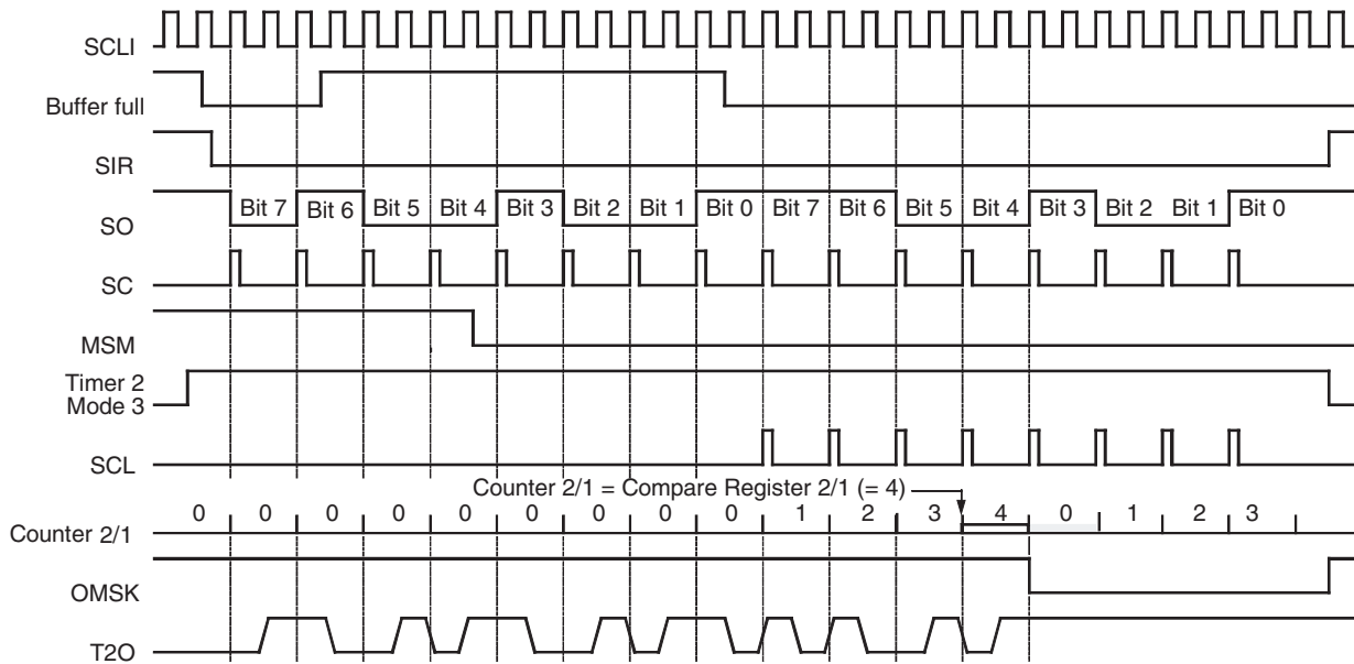
Figure 5-51. Manchester Modulation 2
