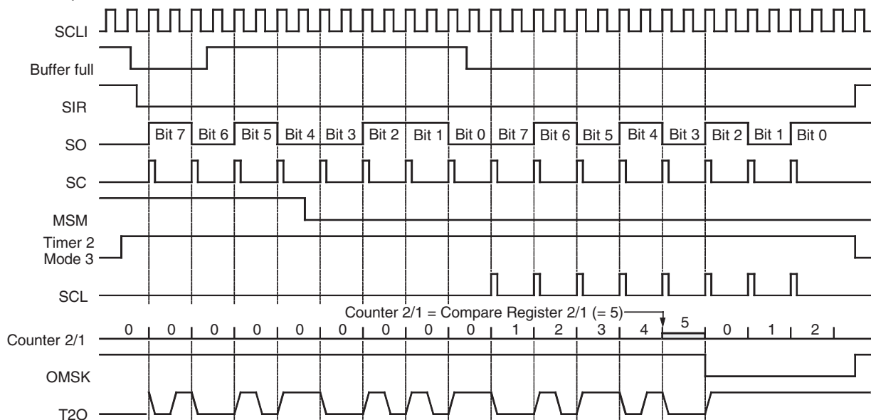
Figure 5-52. Bi-phase Modulation 2
