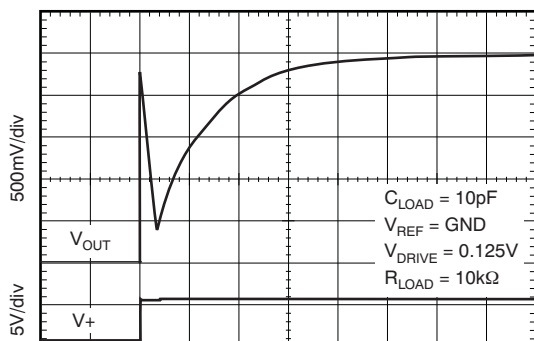
START-UP TRANSIENT RESPONSE
