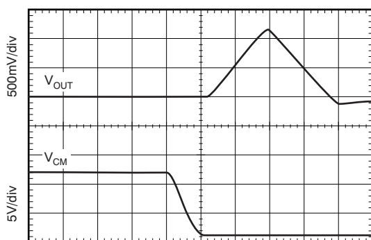
12V COMMON-MODE STEP RESPONSE
