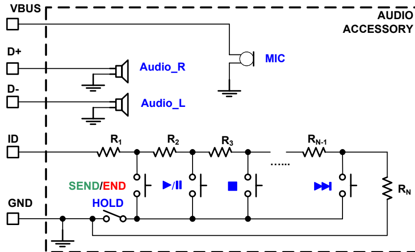
Figure 16. Audio Accessory with Remote Control and Microphone
