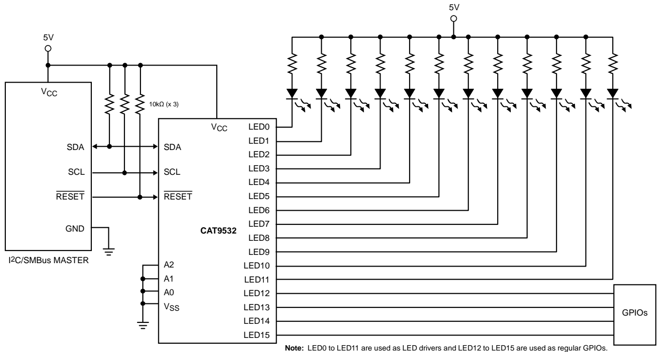
Figure 10. Typical Application
