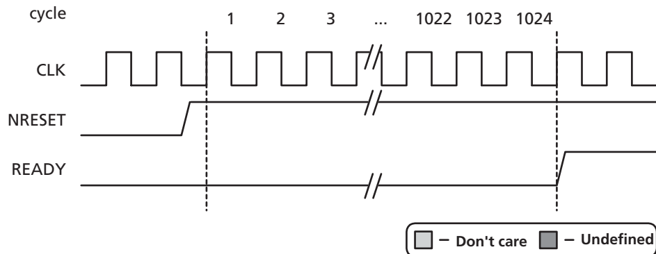
Figure 5 • CoreAES128 Initialization
