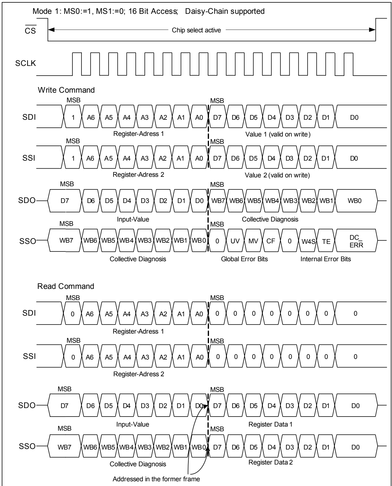
Figure 25 SPI Mode 1
