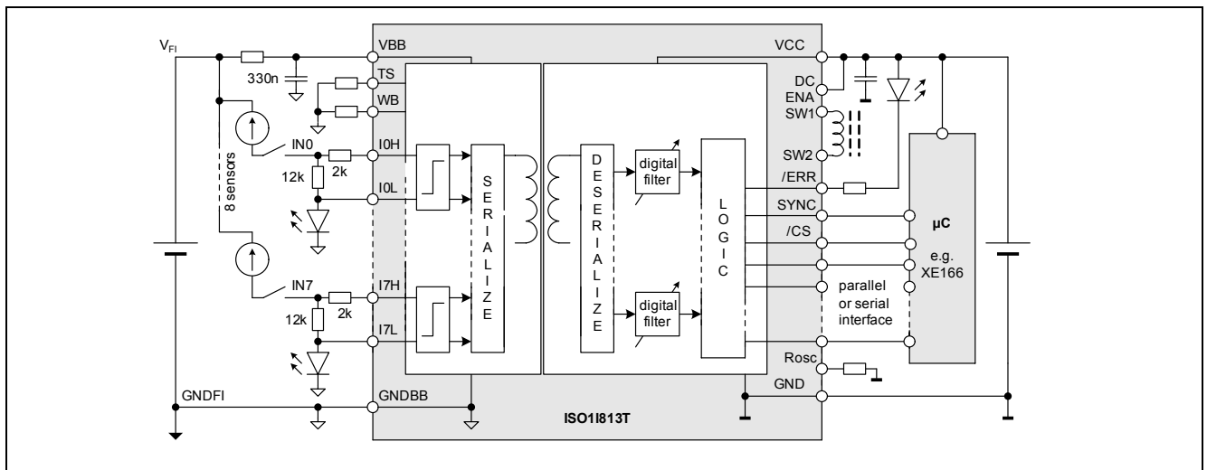
Figure 29 Recommended Application Circuit
