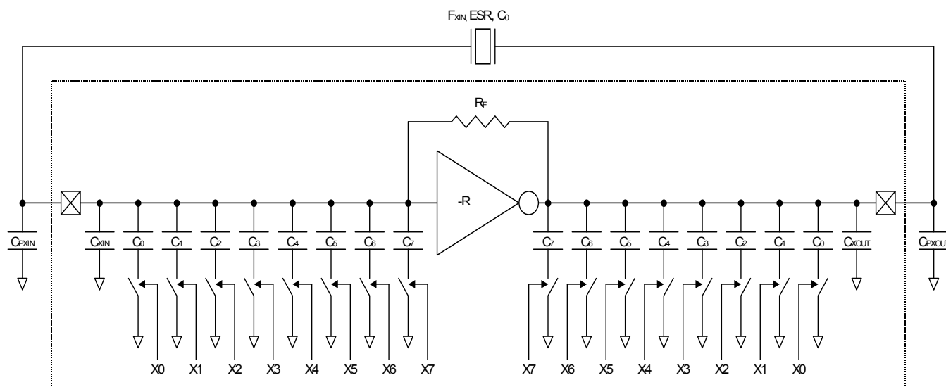
Figure 2. Crystal Oscillator Tuning Block Diagram
