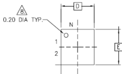
Figure 11. Package Outline Drawing: CY22M1 8-Pin 1.7 x 1.7 x 0.6 mm 3 QFN
