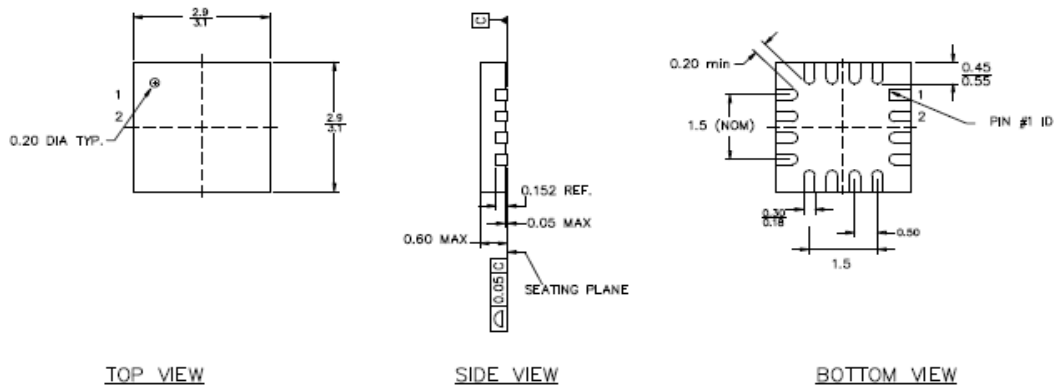
Figure 11. 16-Pin (3x3 mm x 0.6 MAX) COL
