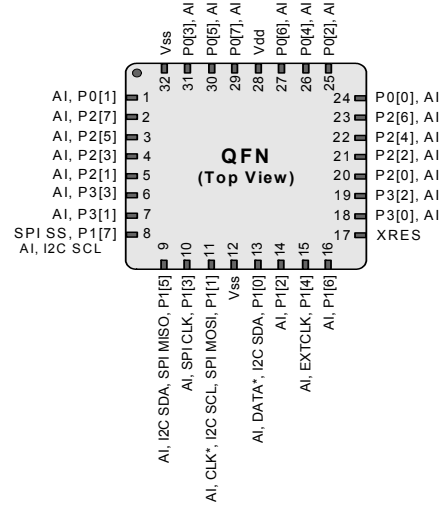
Figure 6. CY8C20424 32-Pin PSoC Device
