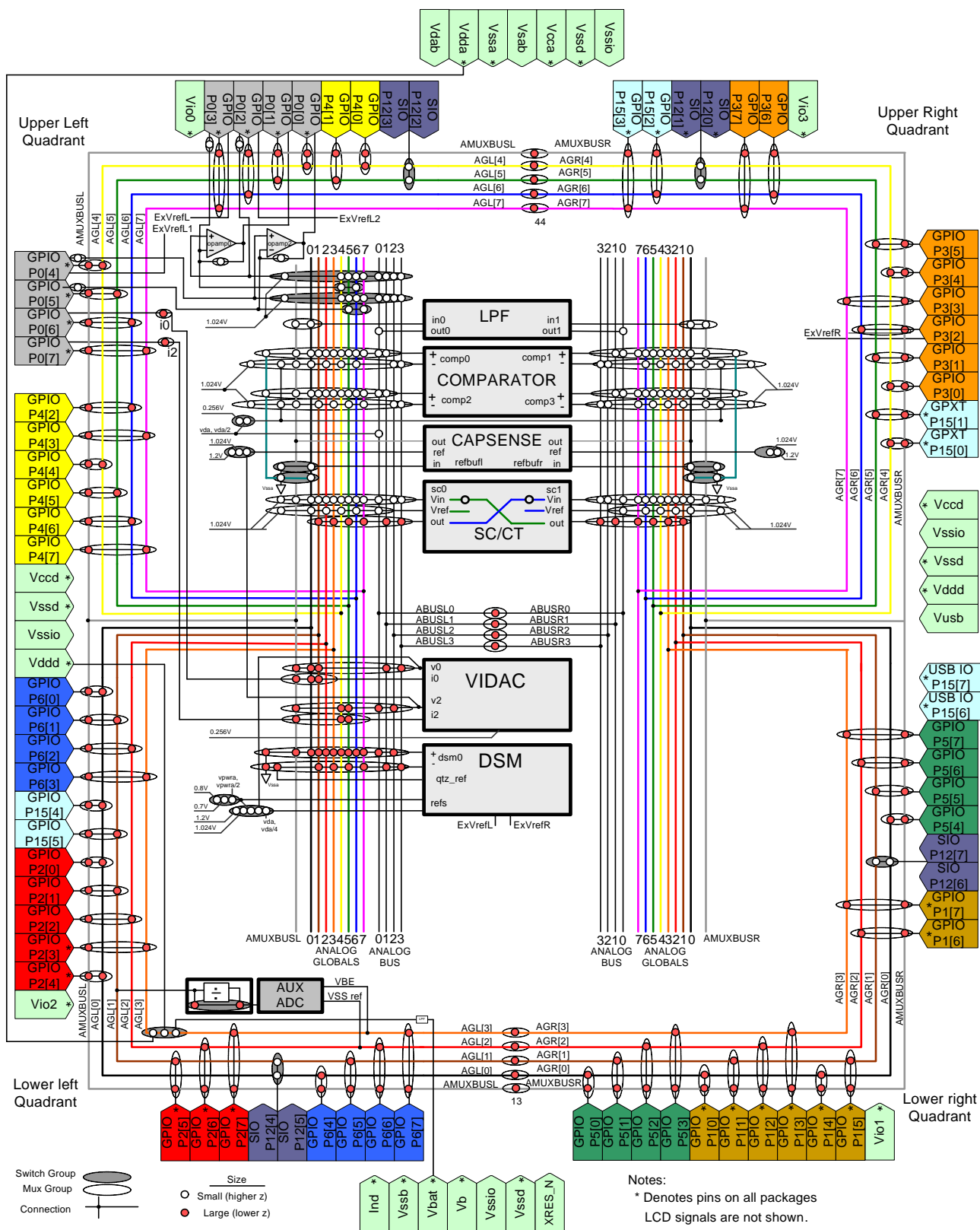
Figure 8-2. CY8C34 Analog Interconnect
