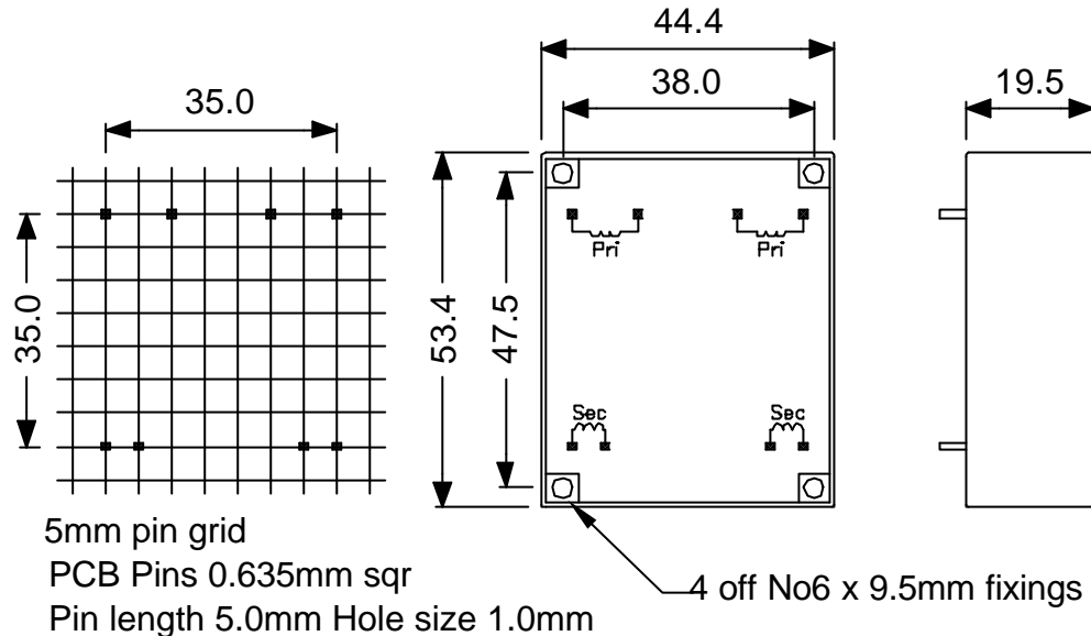
Outline Drawing
