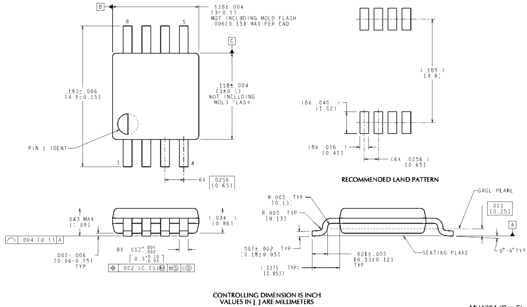
8-Lead MSOP Order Number DAC121S101CIMM NS Package Number MUA08A
