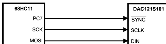
FIGURE 7. 68HC11 Interface
