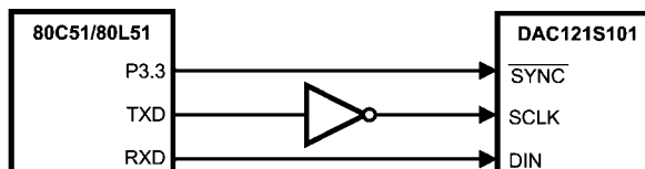
FIGURE 6. 80C51/80L51 Interface
