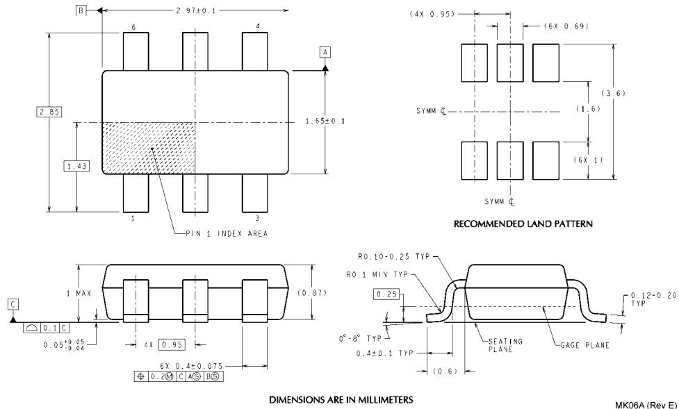
6-Lead TSOT Order Numbers DAC121S101CIMK and DAC121S101QCMK NS Package Number MK06A
