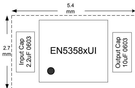
Figure 1: Total Solution Footprint (Not to Scale)
