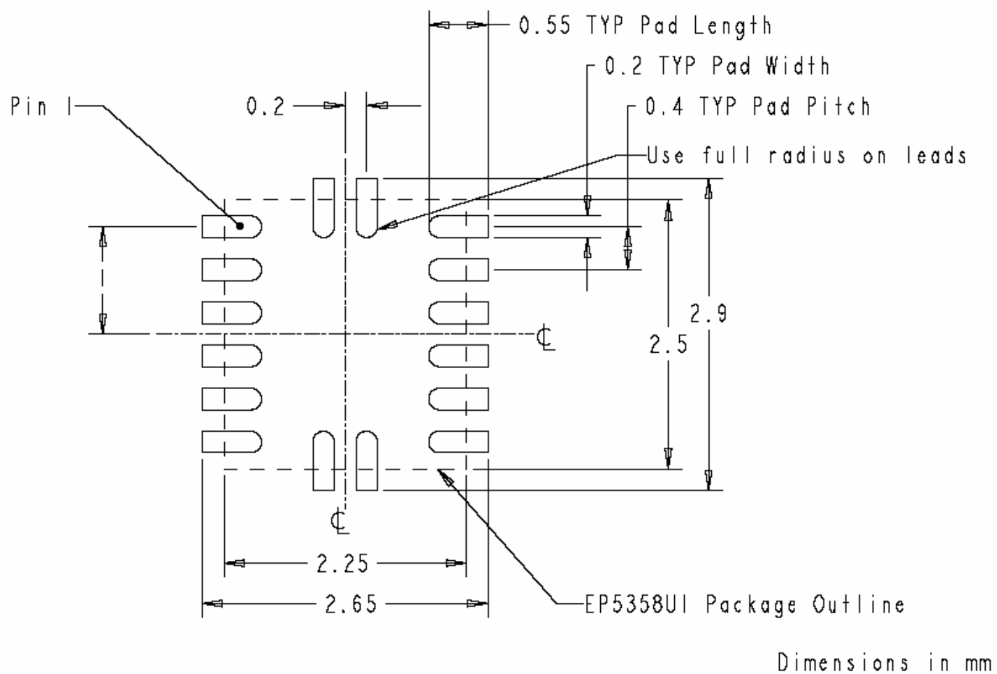
Figure 9: EP5358 Package PCB Footprint
