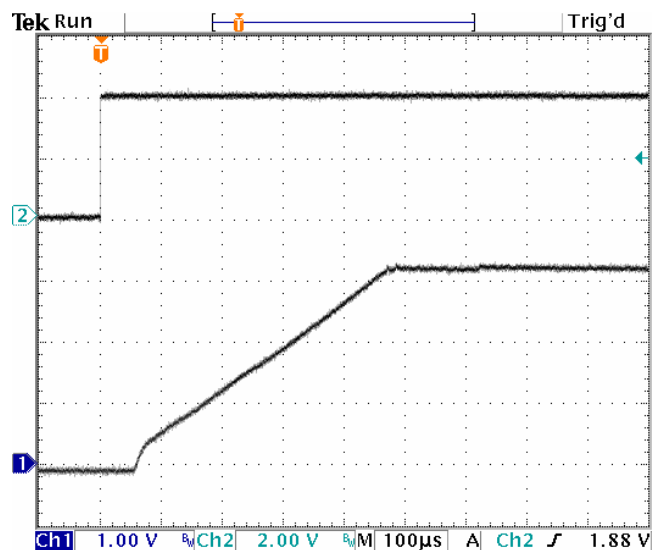
Start Up Waveform: V_{IN} = 5.0V , V_{OUT} = 3.3V ; I_{LOAD} = 10mA
