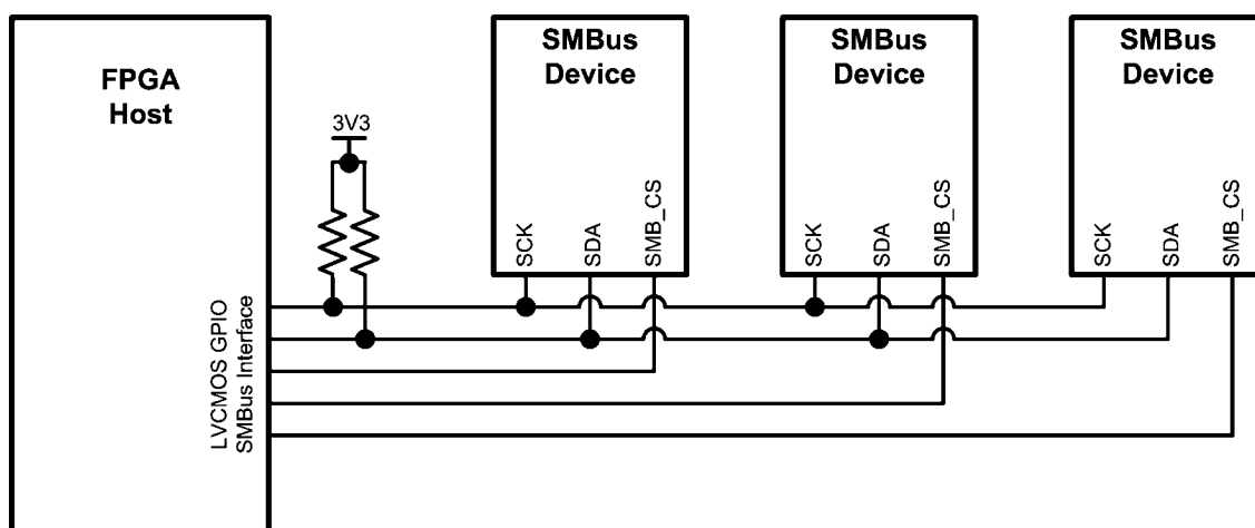
FIGURE 9. SMBus Configuration 2
