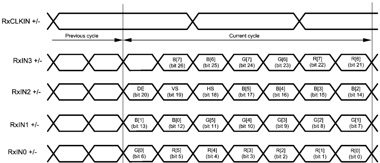
FIGURE 22. 8-bit Channel Link Mapping: MSB's on RxIN3
