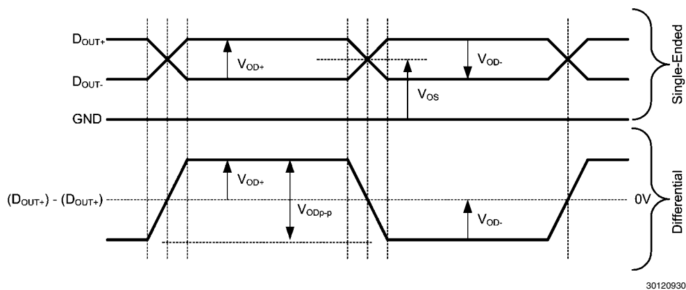
FIGURE 3. Output Waveforms
