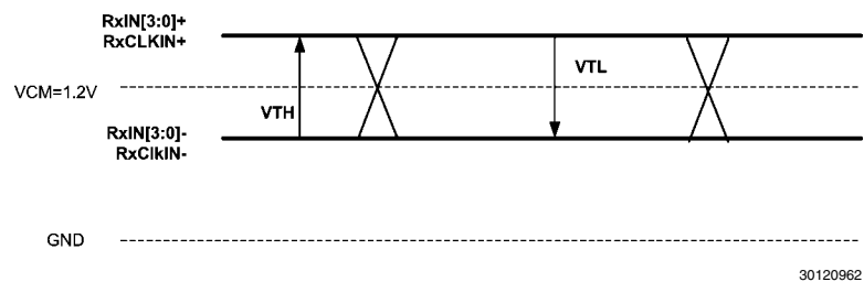
FIGURE 1. Channel Link DC VTH/VTL Definition
