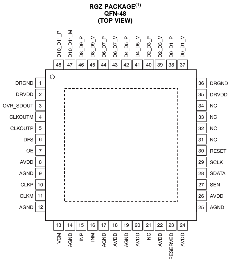
Figure 1. LVDS Pinout
