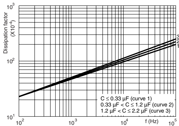
Tanget of loss angle as a function of frequency (typical curve)
