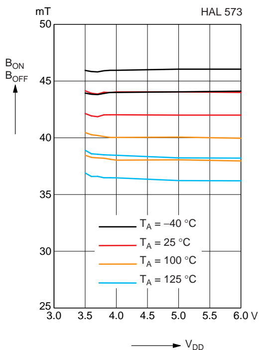
Fig. 4-3: Magnetic switching points versus supply voltage
