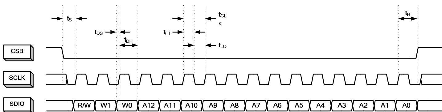
Figure 42. Instruction/Address Phase
