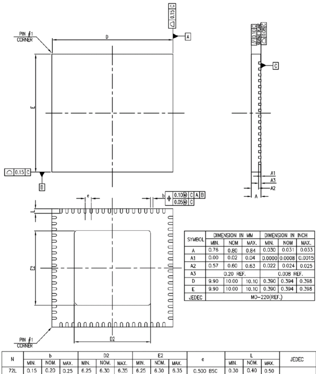
Figure 54. 72QFN Dimensions
