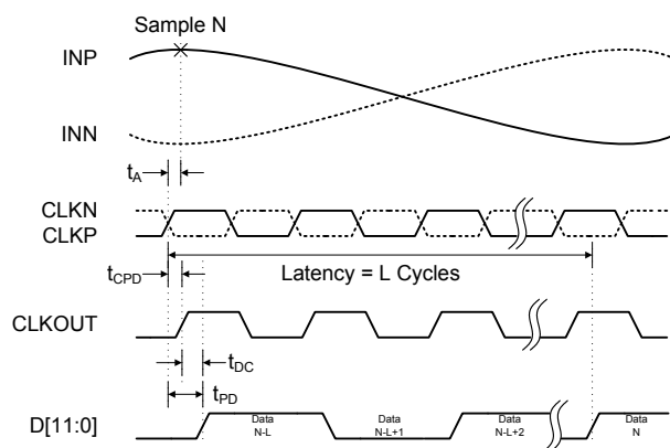
Figure 2b. CMOS Timing Diagram—SDR
