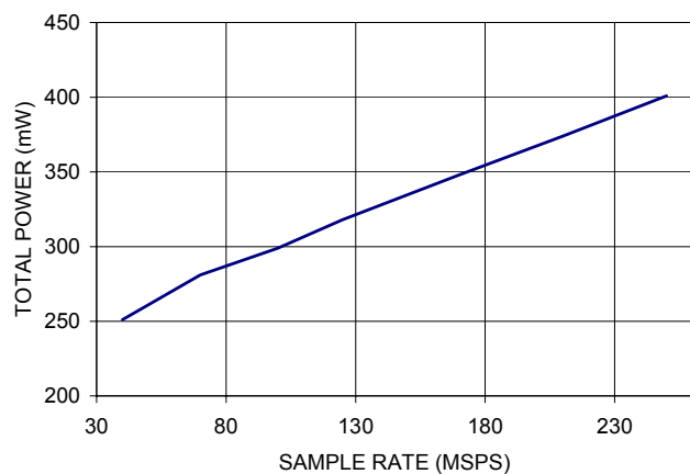
Figure 11. Power vs. f_{\text{SAMPLE}} (LVDS Mode)
