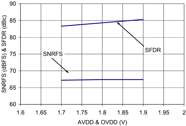
Figure 27. SNR & SFDR vs. Power Supply Voltage
