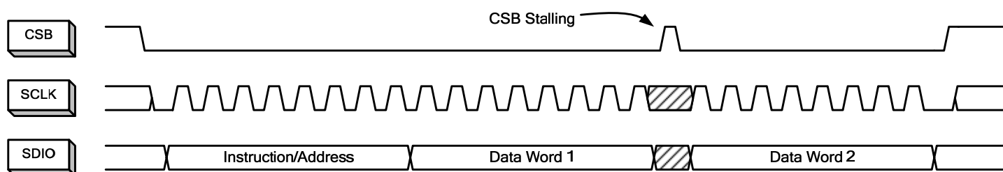
Figure 43. 2-Byte Transfer
