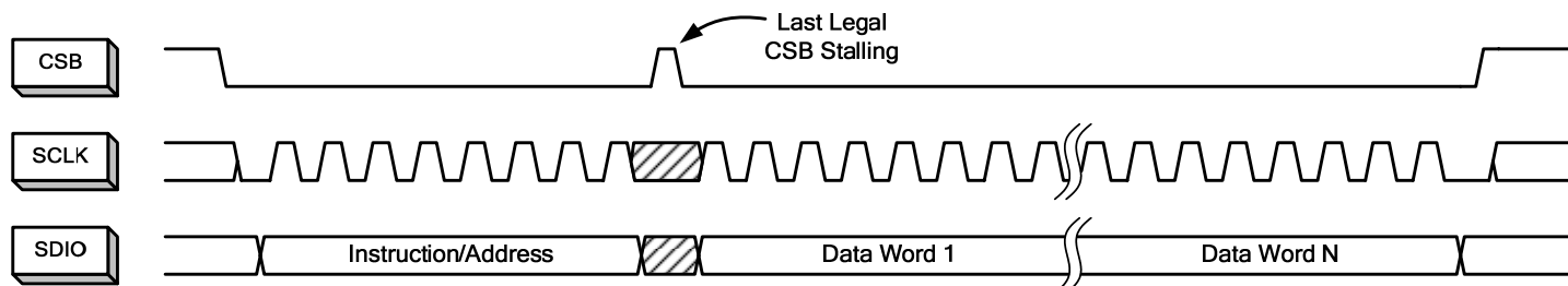
Figure 44. N-Byte Transfer
