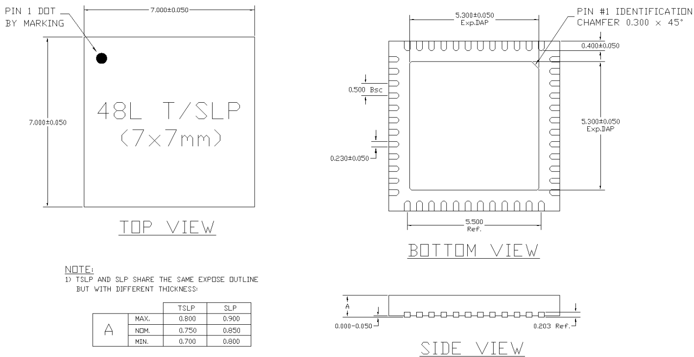
Figure 55. 48QFN Dimensions
