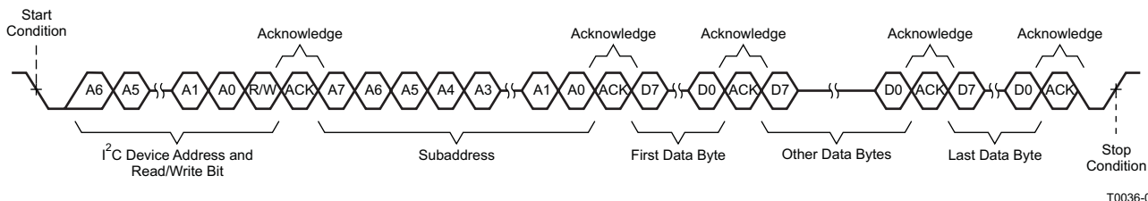
Figure 48. Multiple-Byte Write Transfer
