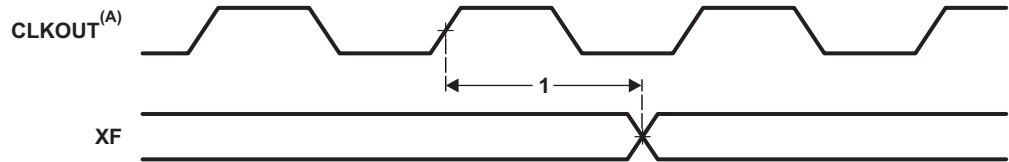
Figure 5-14. XF Timings
