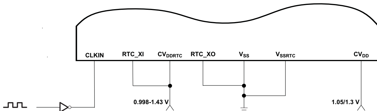
Figure 5-6. LVCMOS-Compatible Clock Input With RTC Oscillator Disabled
