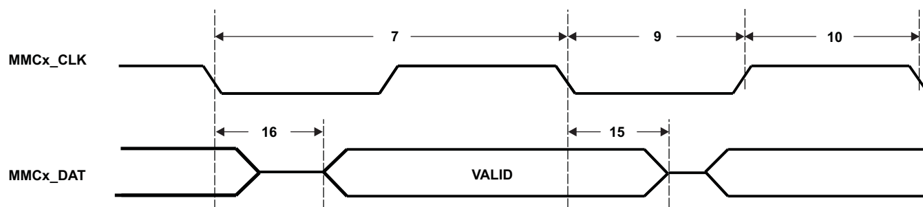
Figure 5-24. MMC/SD Data Write Timing
