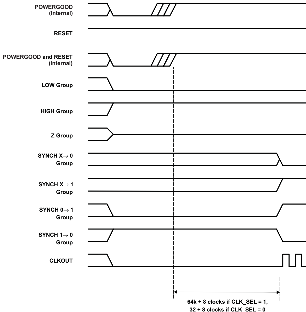
Figure 5-10. Power-On Reset Timing Requirements
