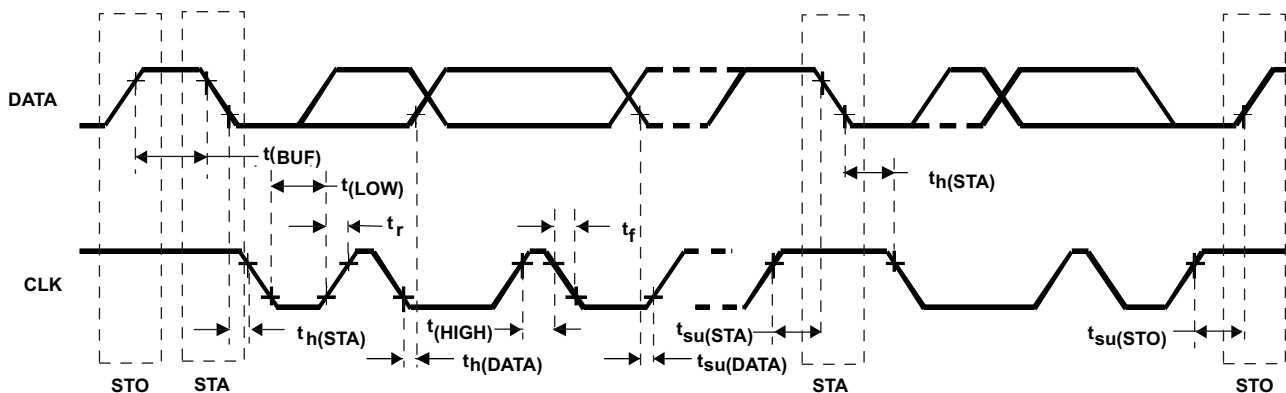
Figure 44. Serial I/f Timing Diagram
