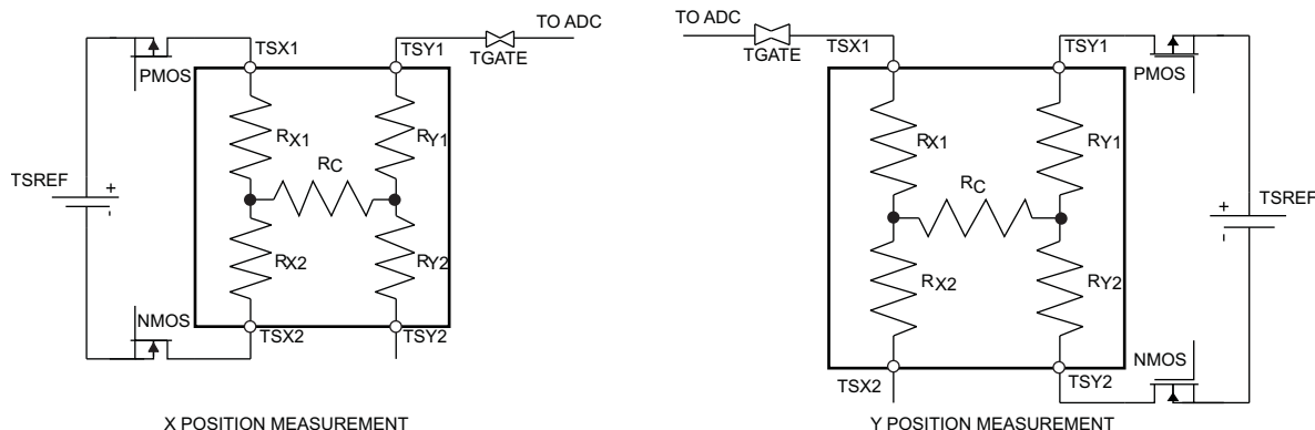
Figure 35. Two Position Measurement
