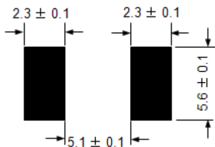
Solder reflow conditions
