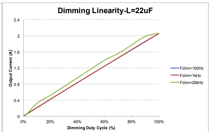
Fig.13 Dimming Linearity of MBI6662: L=22uH
