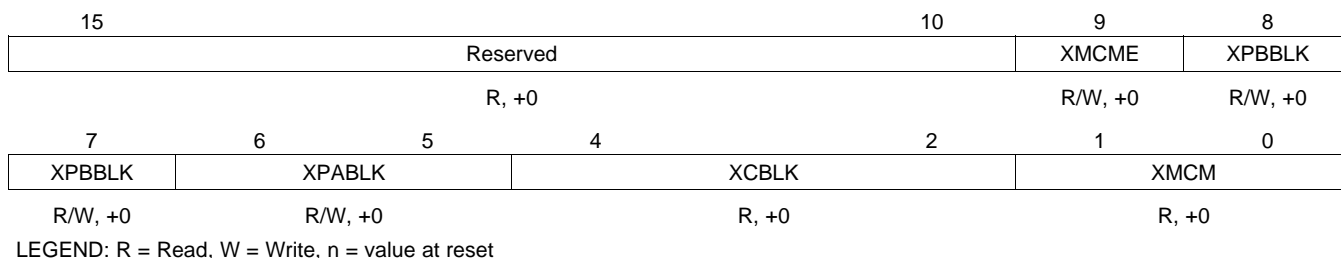
Figure 3-12. Multichannel Control Register 2x (MCR2x)
