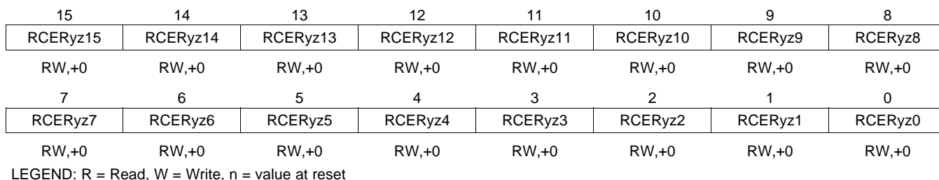
Figure 3-13. Receive Channel Enable Registers Bit Layout for Partitions A to H
