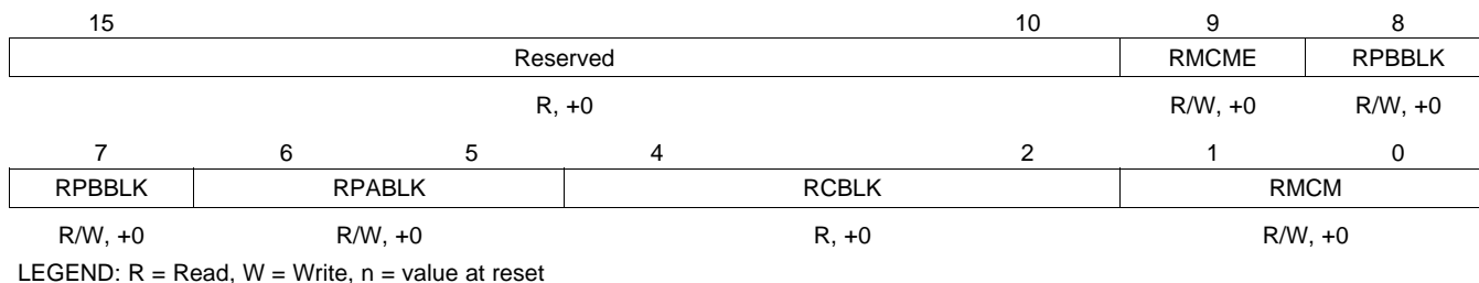
Figure 3-11. Multichannel Control Register 1x (MCR1x)
