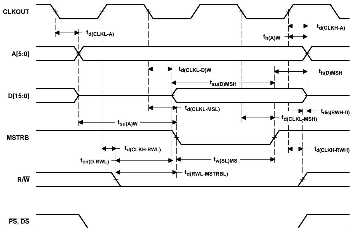
Figure 6–6. Memory Write
