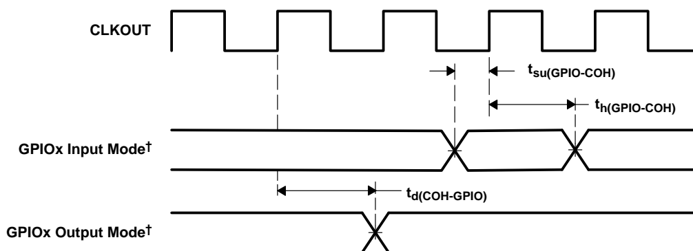
Figure 6-30. GPIOx † Timings
