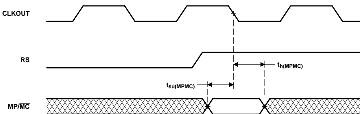
Figure 6-16. MP/MC Timing
