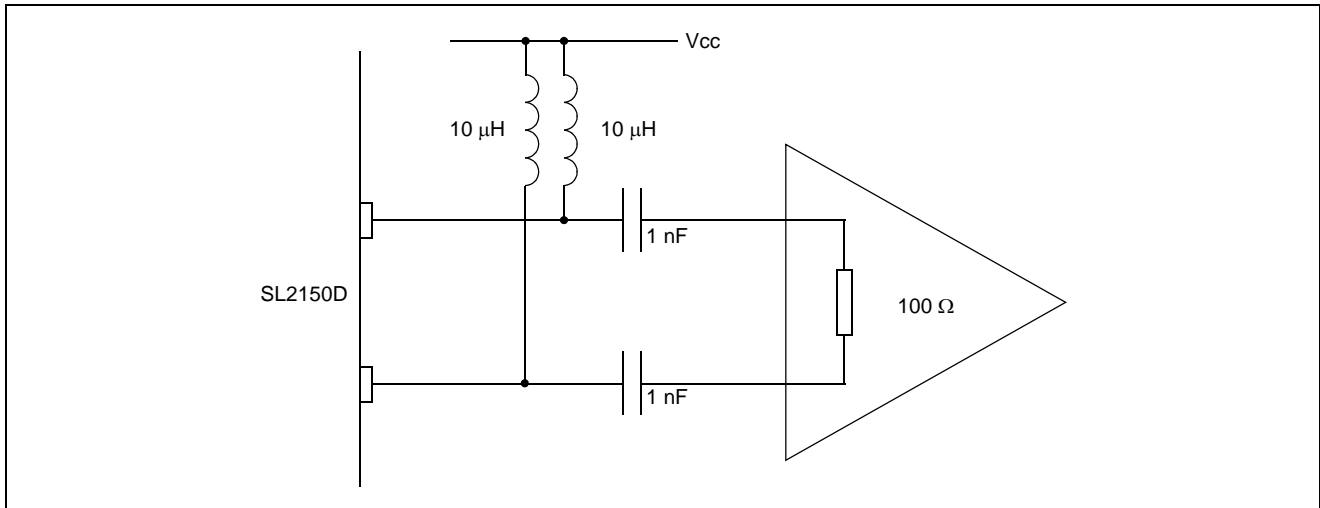
Figure 12 - Example Application Driving 100 \Omega Load with Inductive Pull Up
