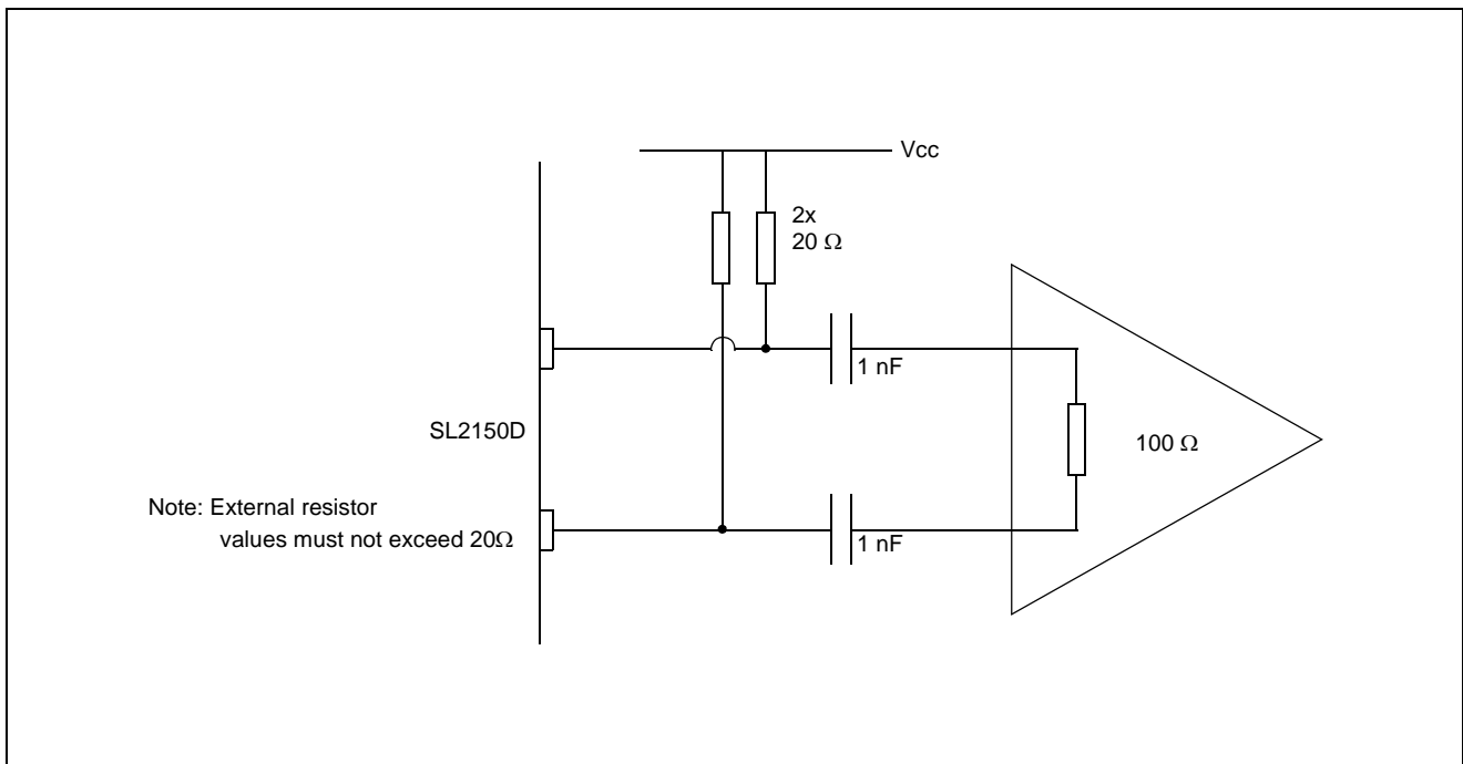
Figure 13 - Example Application Driving 100 \Omega Load with Resistive Pull Up
