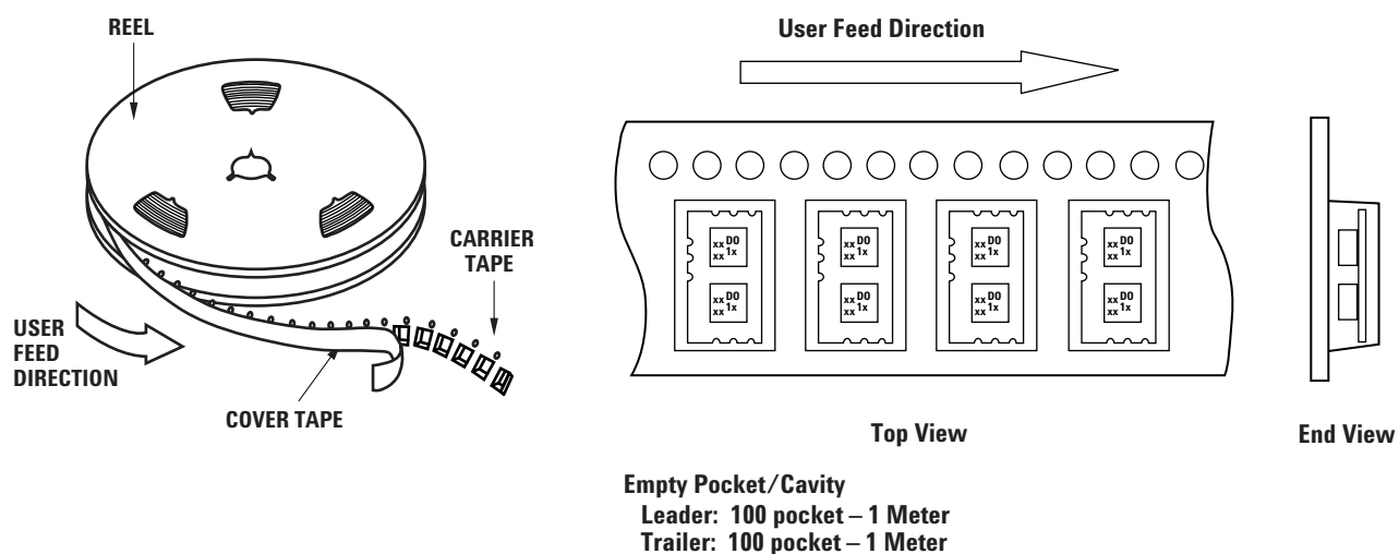
Figure 15. Device Orientation.
