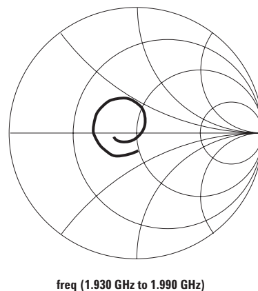
Figure 6. S_{22} , Rx Port Impedance (typical).
