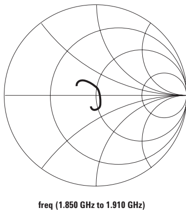
Figure 5. S_{11} , Tx Port Impedance (typical).
