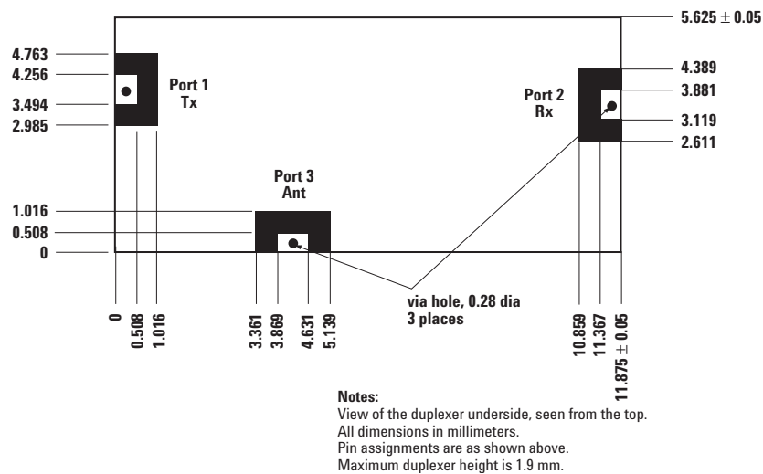
Figure 12. Outline Drawing.
