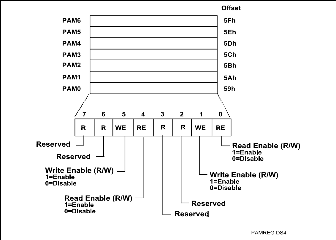
Figure 8. PAM Registers
