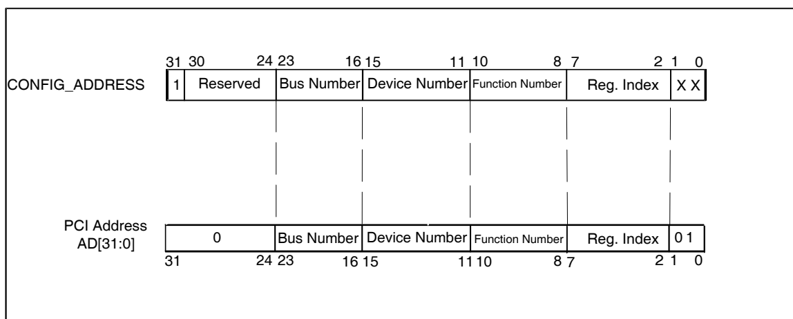
Figure 7. Mechanism #1 Type 1 Configuration Address to PCI Address Mapping
