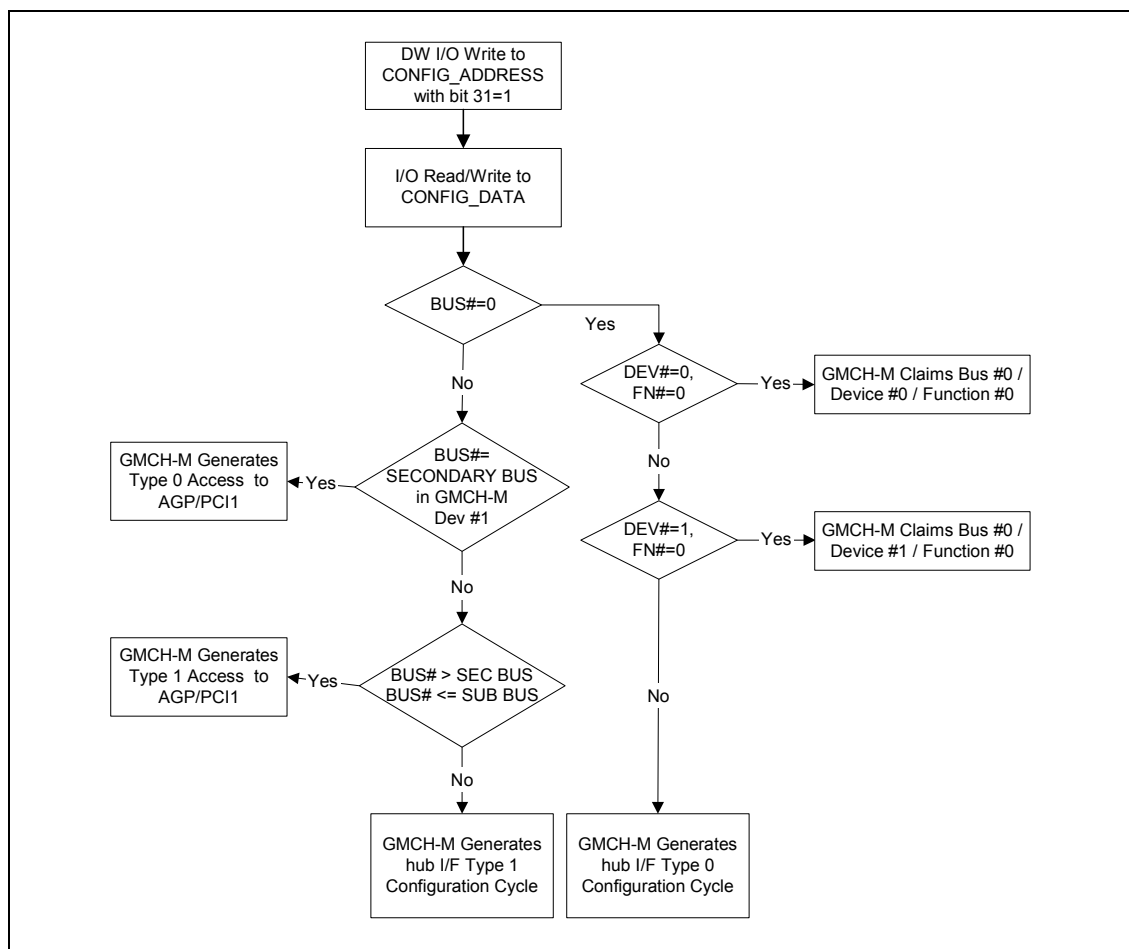
Figure 3. Configuration Cycle Flow Chart
