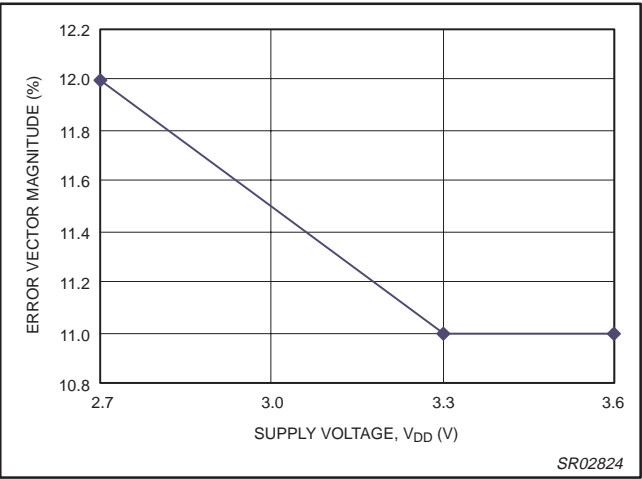
Figure 21. Transmitter error vector magnitude (EVM) versus supply voltage ( T_{\text{amb}} = 25^\circ\text{C} ).
