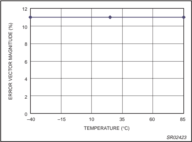
Figure 20. Transmitter error vector magnitude (EVM) versus temperature ( V_{\text{DD}} = 3.3\text{ V} ).
