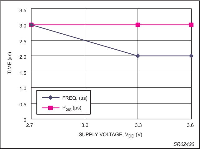
Figure 23. RX to TX switching time versus supply voltage ( T_{\text{amb}} = 25^\circ\text{C} ).
