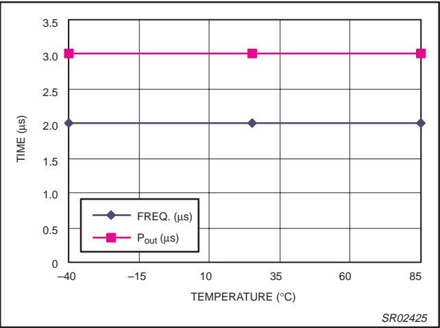
Figure 22. RX to TX switching time versus temperature ( V_{\text{DD}} = 3.3\text{ V} ).
