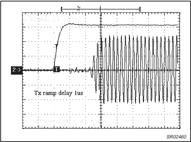
Figure 18. TX ramp-up (1 \mu\text{s}/\text{div} ).
