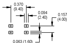
SUGGESTED SOLDER PAD LAYOUT
