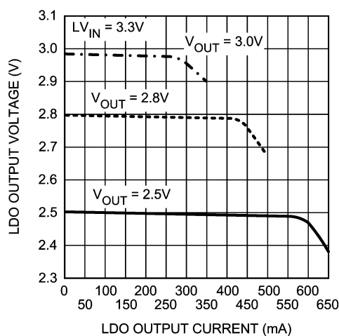
LDO V_{OUT} vs. Load Current
