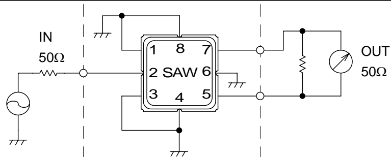
Fig.1 Measuring circuit
