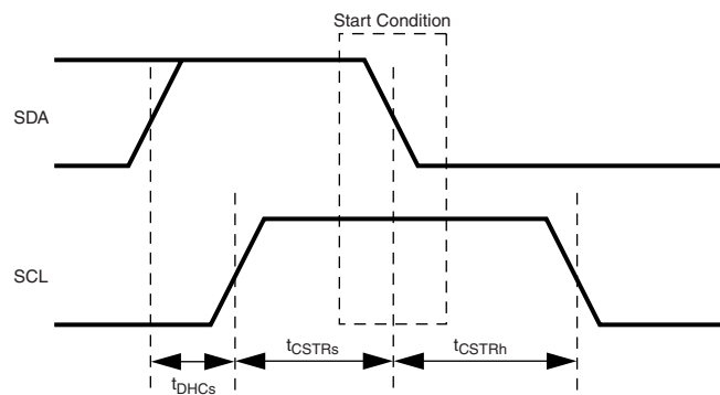
Figure 87. ACB Start and Stop Condition Timing
