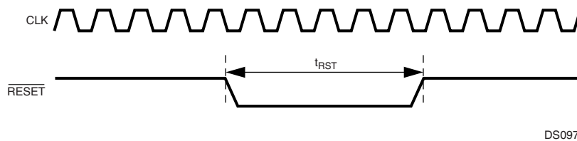
Figure 74. Non-Power-On Reset
