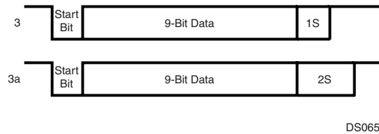
Figure 45. 9-bit Data Frame Options
