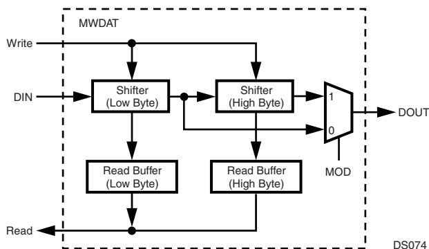
Figure 54. MWDAT Register
