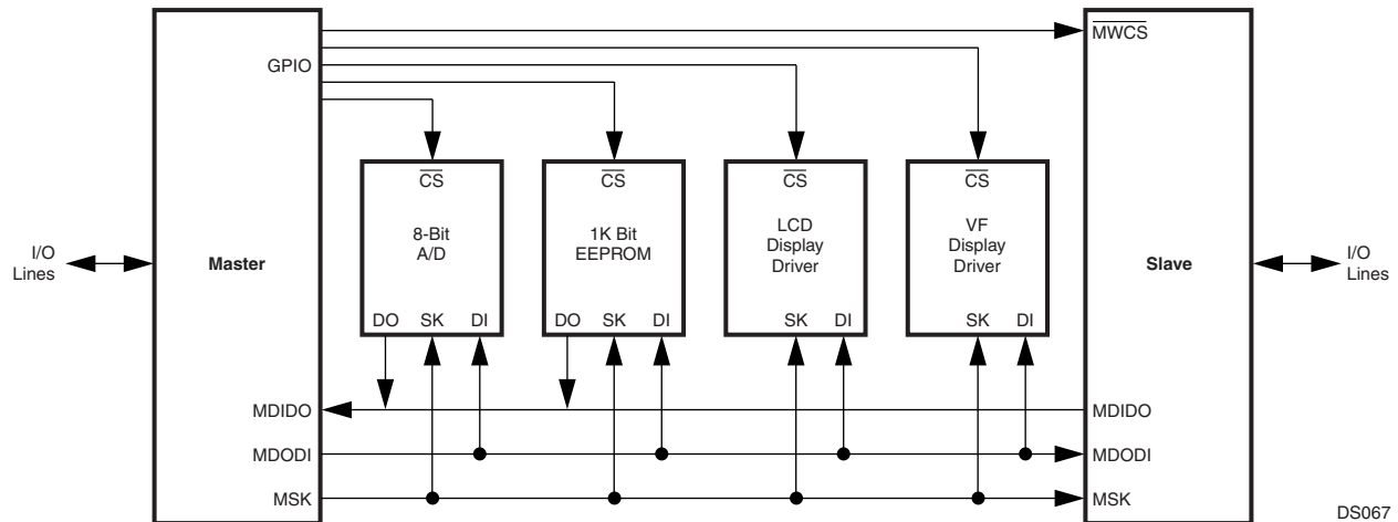
Figure 47. Microwire Interface
