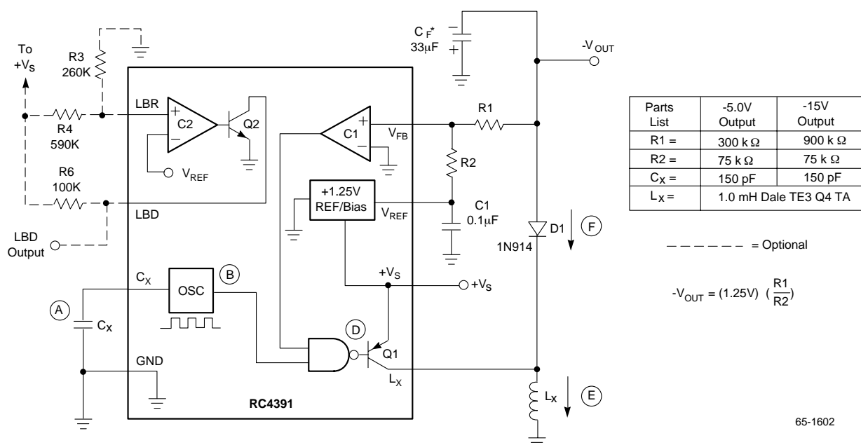
Figure 8. Inverting Regulator – Standard Circuit
