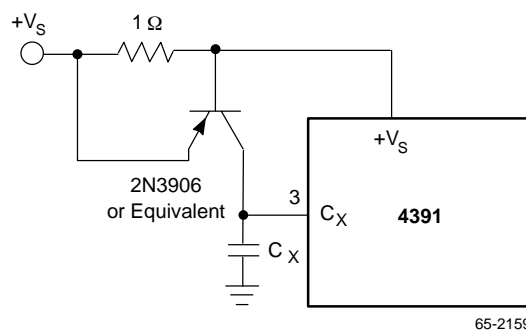
Figure 18. Current Limiting
