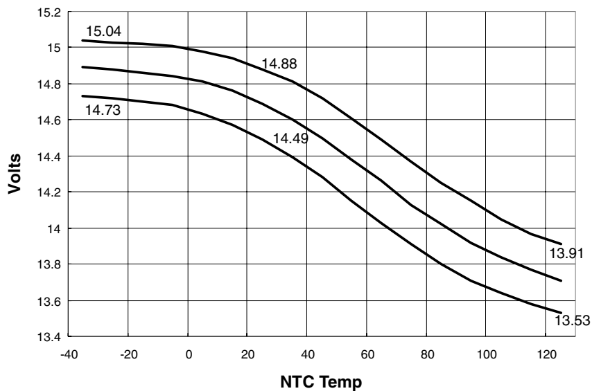
Figure 5. Set-Point Voltage vs. Thermistor Temperature, T_j = 90^\circ\text{C} (Not guaranteed by testing, depending on NTC characteristics)
