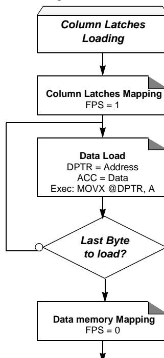
Figure 17. Column Latches Loading Procedure
