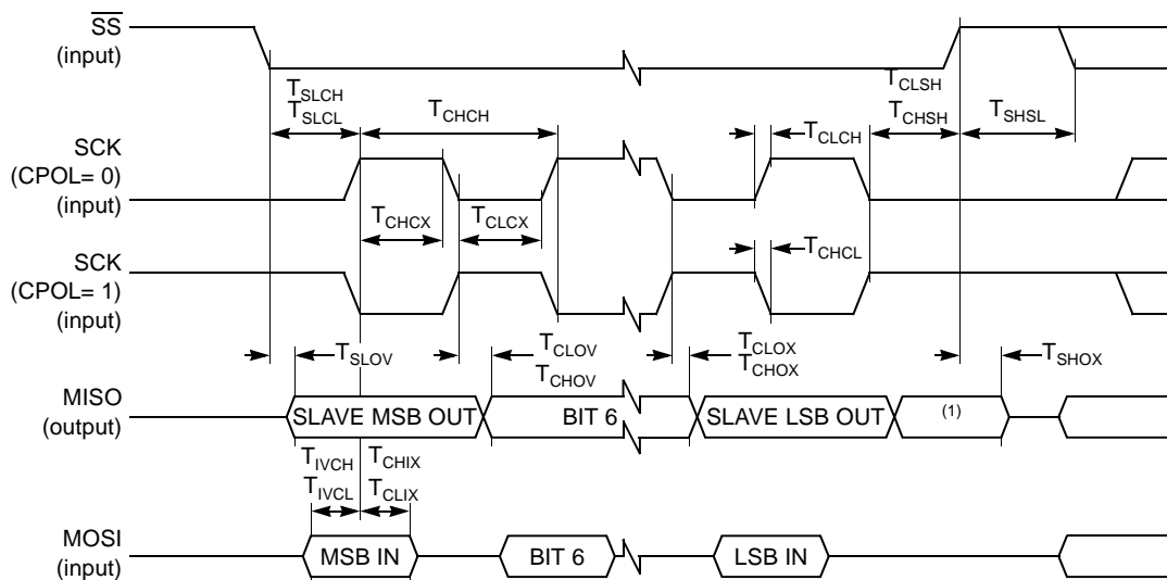
Figure 83. SPI Slave Waveforms (CPHA= 0)
