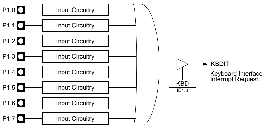
Figure 40. Keyboard Input Circuitry
