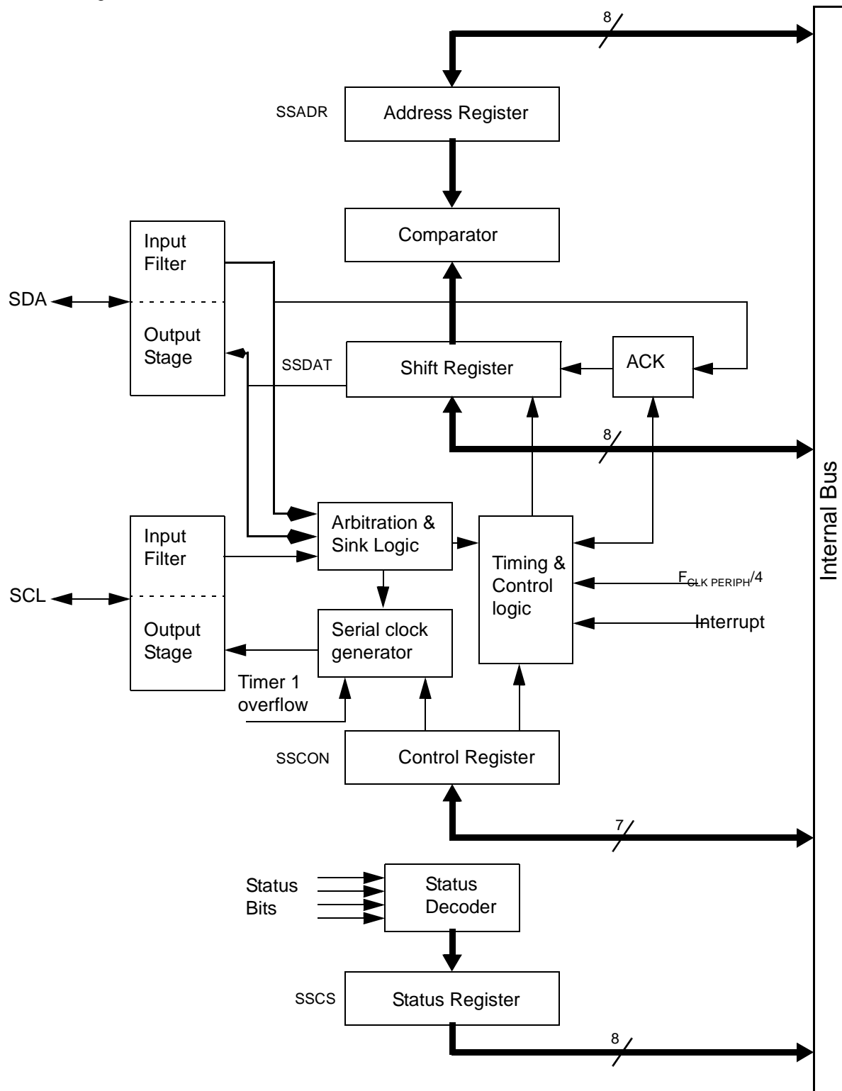
Figure 49. Block Diagram
