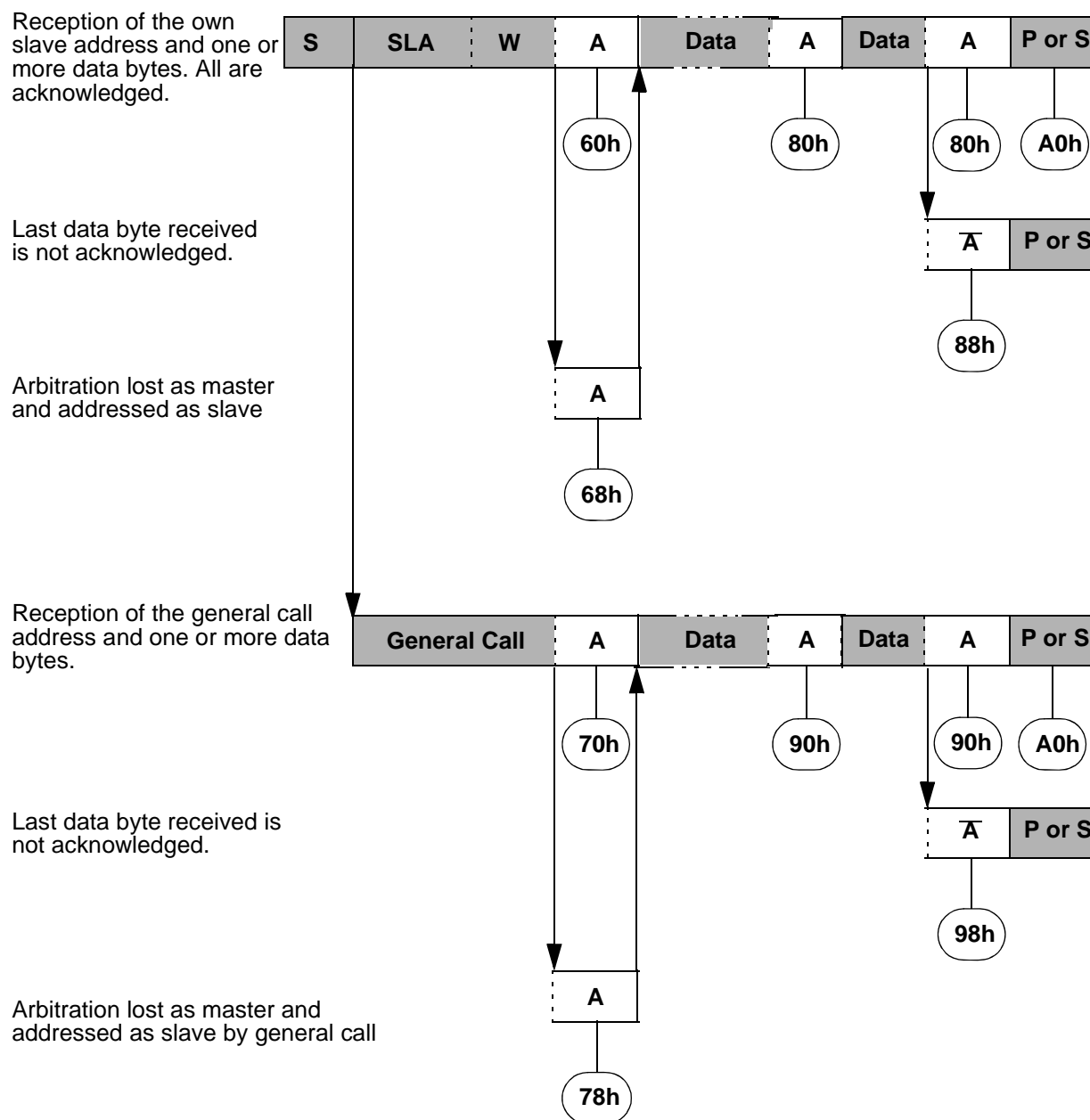
Figure 53. Format and State in the Slave Receiver Mode
