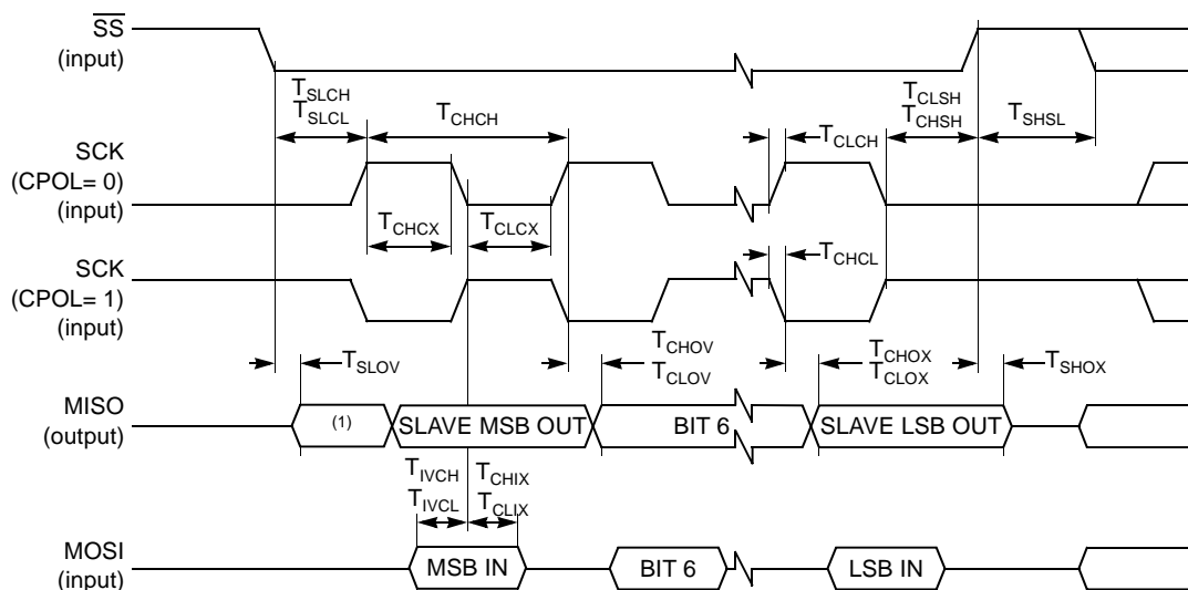
Figure 84. SPI Slave Waveforms (CPHA= 1)
