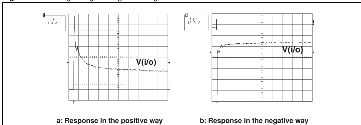
Fig. A4: Remaining voltage during ESD surge.
